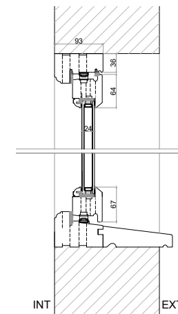
W-018 - Timber D/G Proposed Section A Scale 1/10
