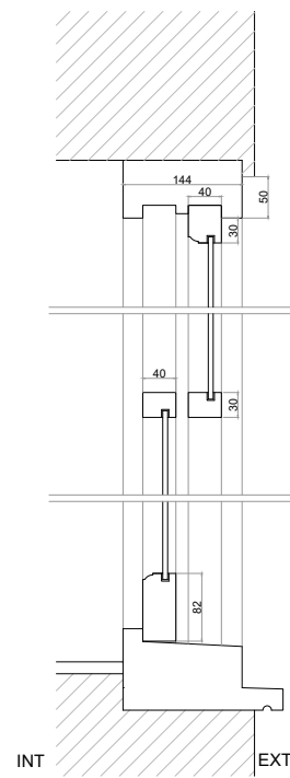
W-020 - Timber S/G Existing Section A Scale 1/10
