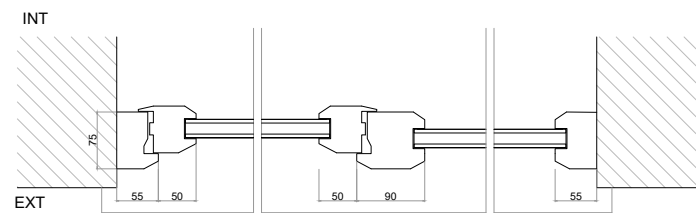
W-021 - PVC D/G Existing Section B Scale 1/10
