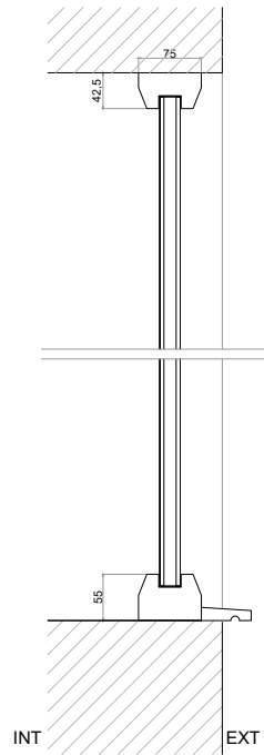
W-017 - PVC D/G Existing Section A Scale 1/10
