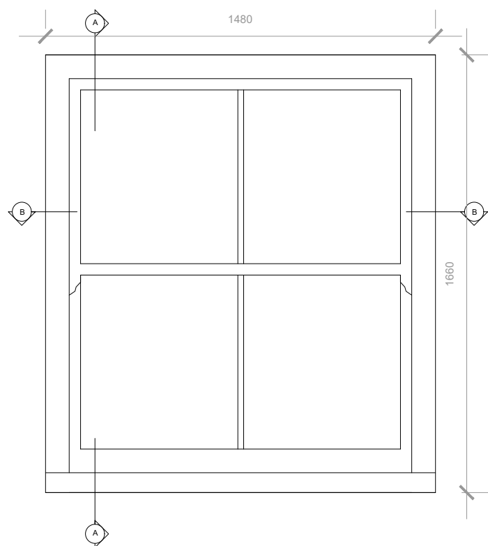
W-021 PROPOSED ELEVATION Scale 1/20
