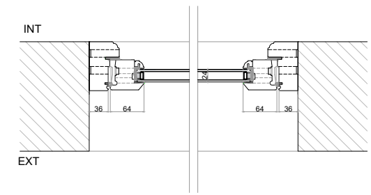
W-019 - Timber D/G Proposed Section B Scale 1/10
