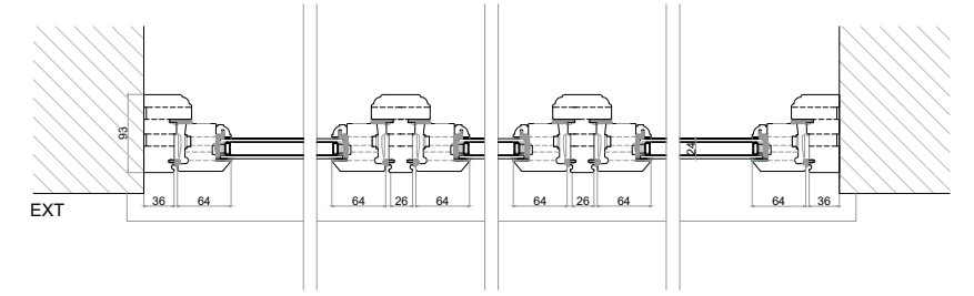
W-016 - Timber D/G Proposed Section B Scale 1/10
