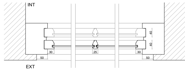
W-020-Timber S/G Existing Section B Scale 1/10
