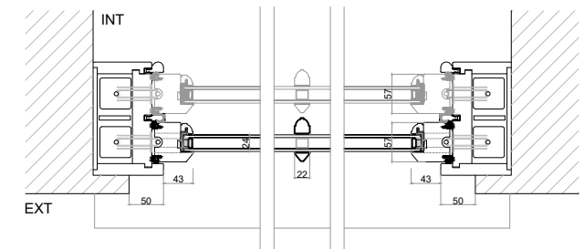
W-020-Timber D/G Proposed Section B Scale 1/10
