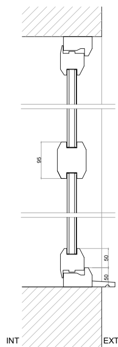
W-021- PVC D/G Existing Section A Scale 1/10
