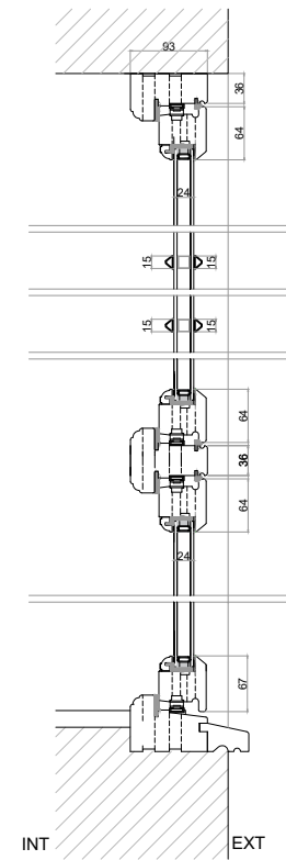
W-016 - Timber D/G Proposed Section A Scale 1/10
