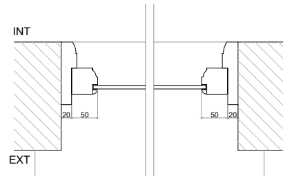
W-018 - Timber S/G Existing Section B Scale 1/10
