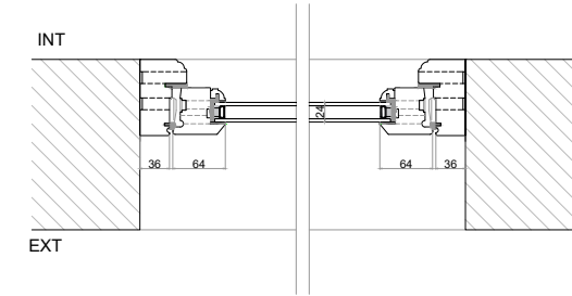
W-018 - Timber D/G Proposed Section B Scale 1/10
