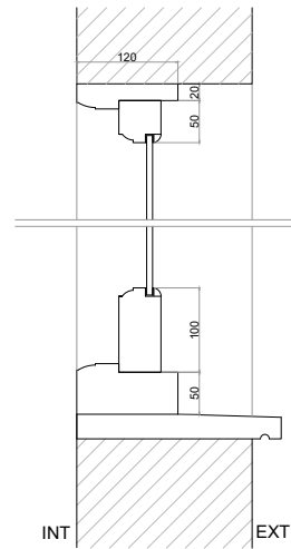
W-018 - Timber S/G Existing Section A Scale 1/10
