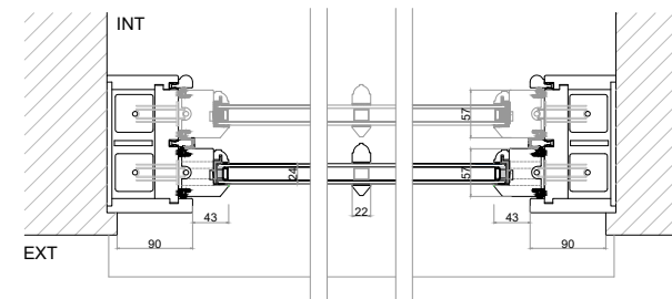
W-021-Timber D/G Proposed Section B Scale 1/10
