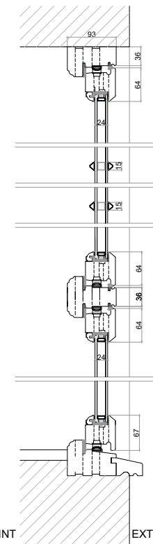
W-017 - Timber D/G Proposed Section A Scale 1/10
