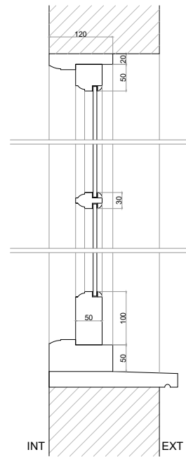
W-019 - Timber S/G Existing Section A Scale 1/10
