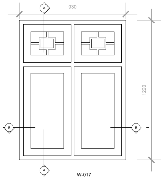
W-017 PROPOSED ELEVATION Scale 1/20
