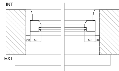
W-019 - Timber S/G Existing Section B Scale 1/10
