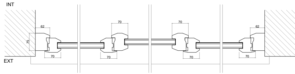
W-016 - PVC D/G Existing Section B Scale 1/10
