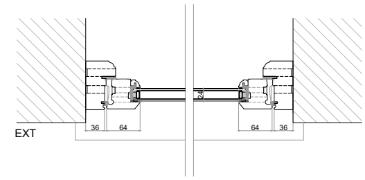
W-017 - Timber D/G Proposed Section B Scale 1/10
