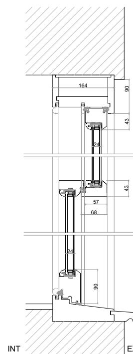
W-021 - Timber D/G Proposed Section A Scale 1/10
