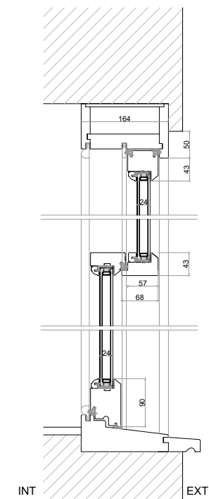
W-020 - Timber D/G Proposed Section A Scale 1/10
