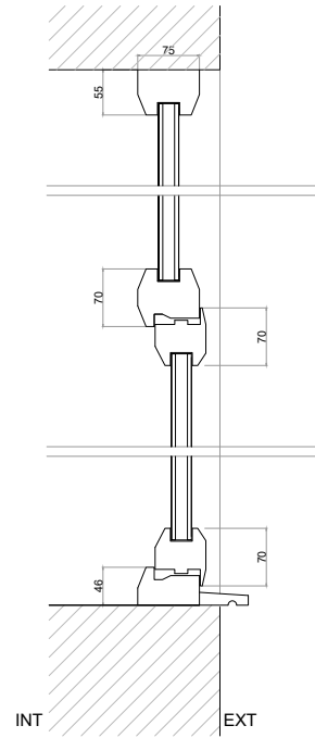
W-016 - PVC D/G Existing Section A Scale 1/10
