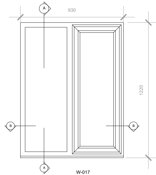
W-017 EXISTING ELEVATION Scale 1/20
