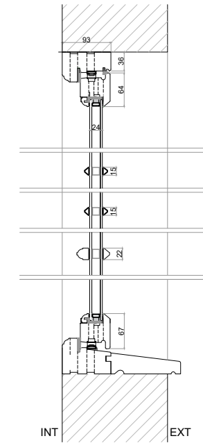
W-019 - Timber D/G Proposed Section A Scale 1/10
