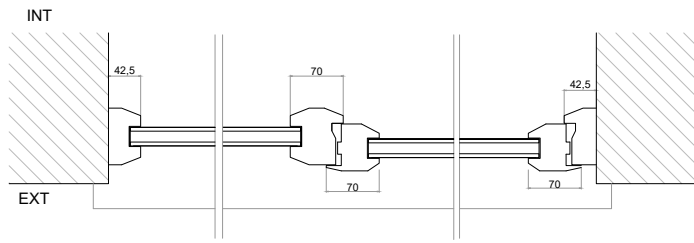
W-017 - PVC D/G Existing Section B Scale 1/10
