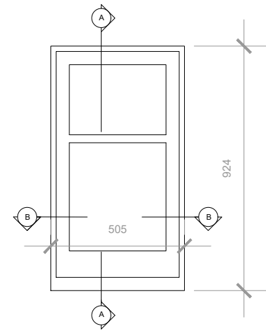
W-019 EXISTING ELEVATION Scale 1/20
