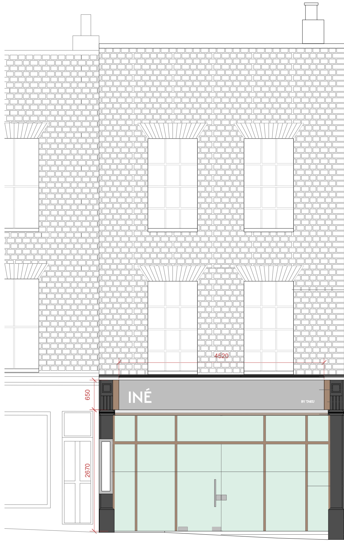
PROPOSED FACADE DESIGN 1:50
