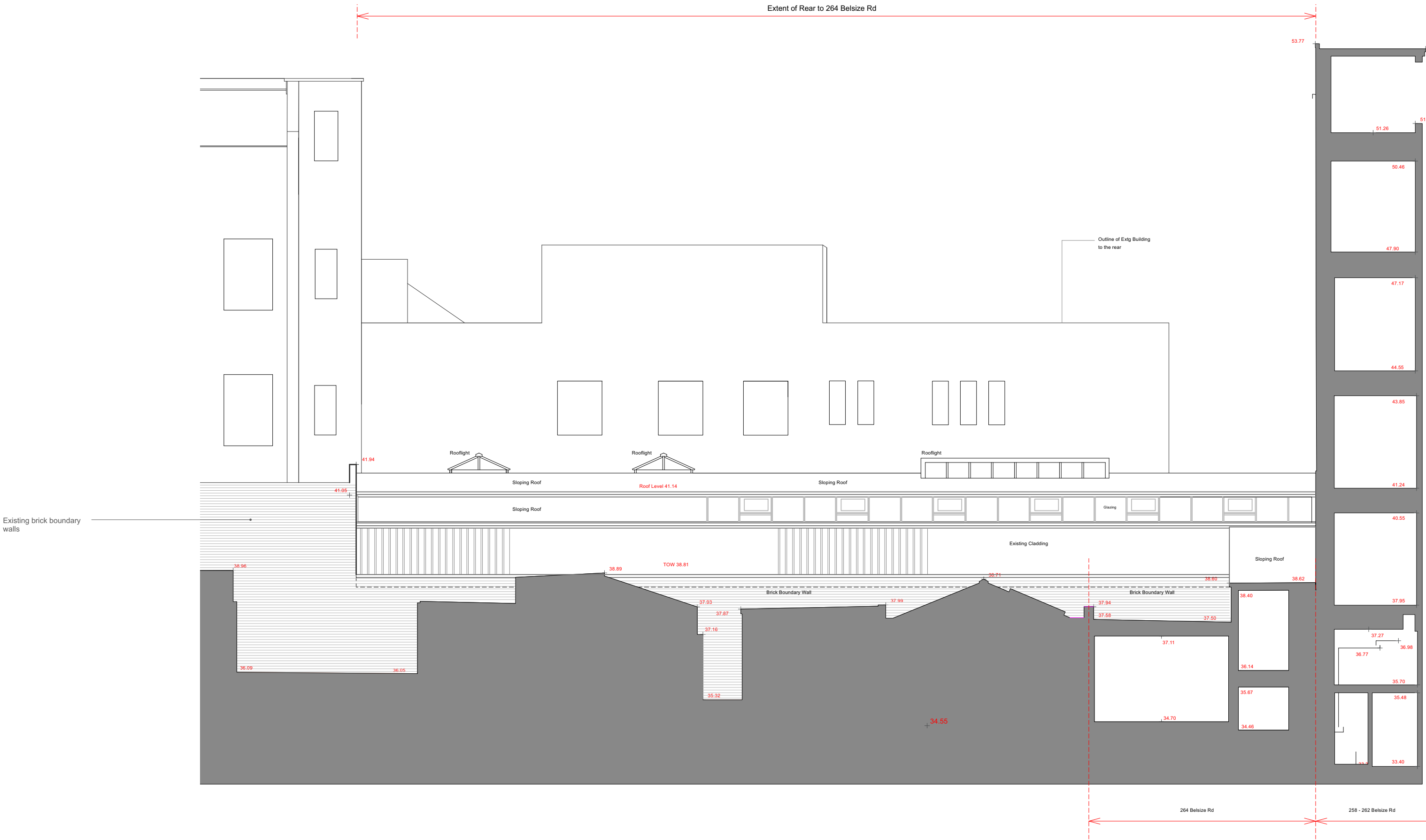
SECTIONAL ELEVATION D-D
