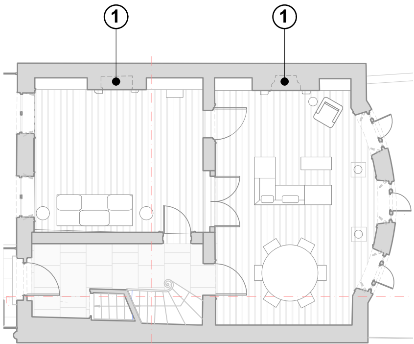
1 Proposed Ground Floor Plan 604 NTS@A3
