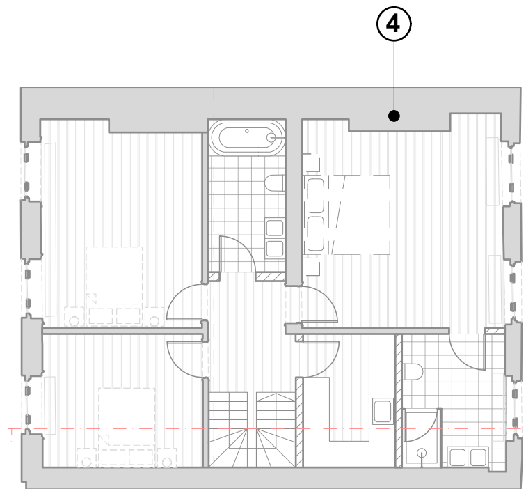
3 Proposed Second Floor Plan 604 NTS@A3
