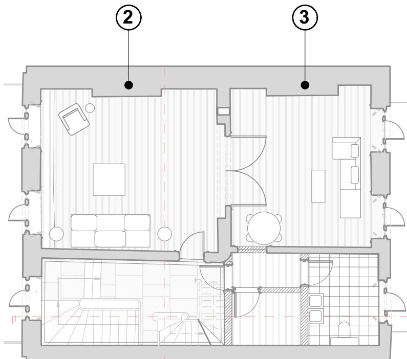
2 Proposed First Floor Plan 604 NTS@A3
