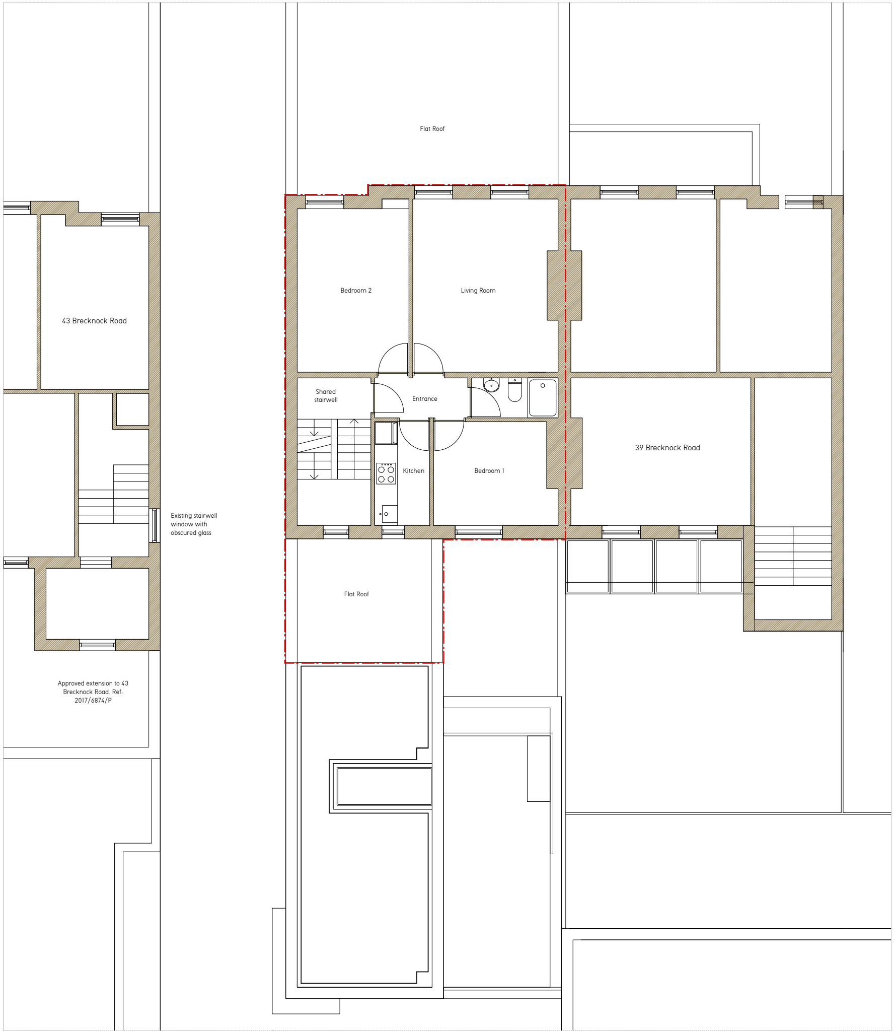
1 Proposed First Floor Plan
