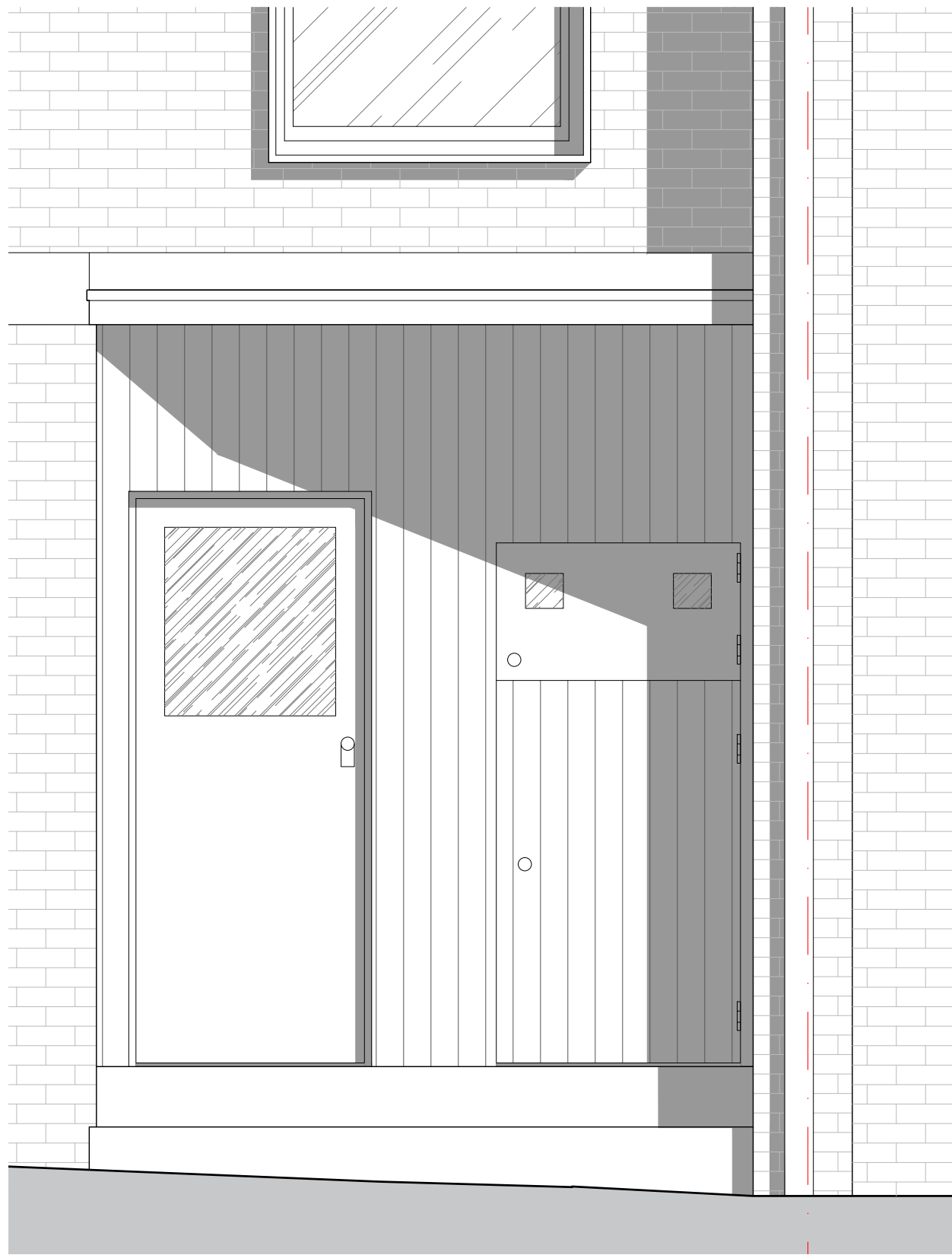
Existing Rear Door and Panelling to No 41 Scale 1:20 @ A3
