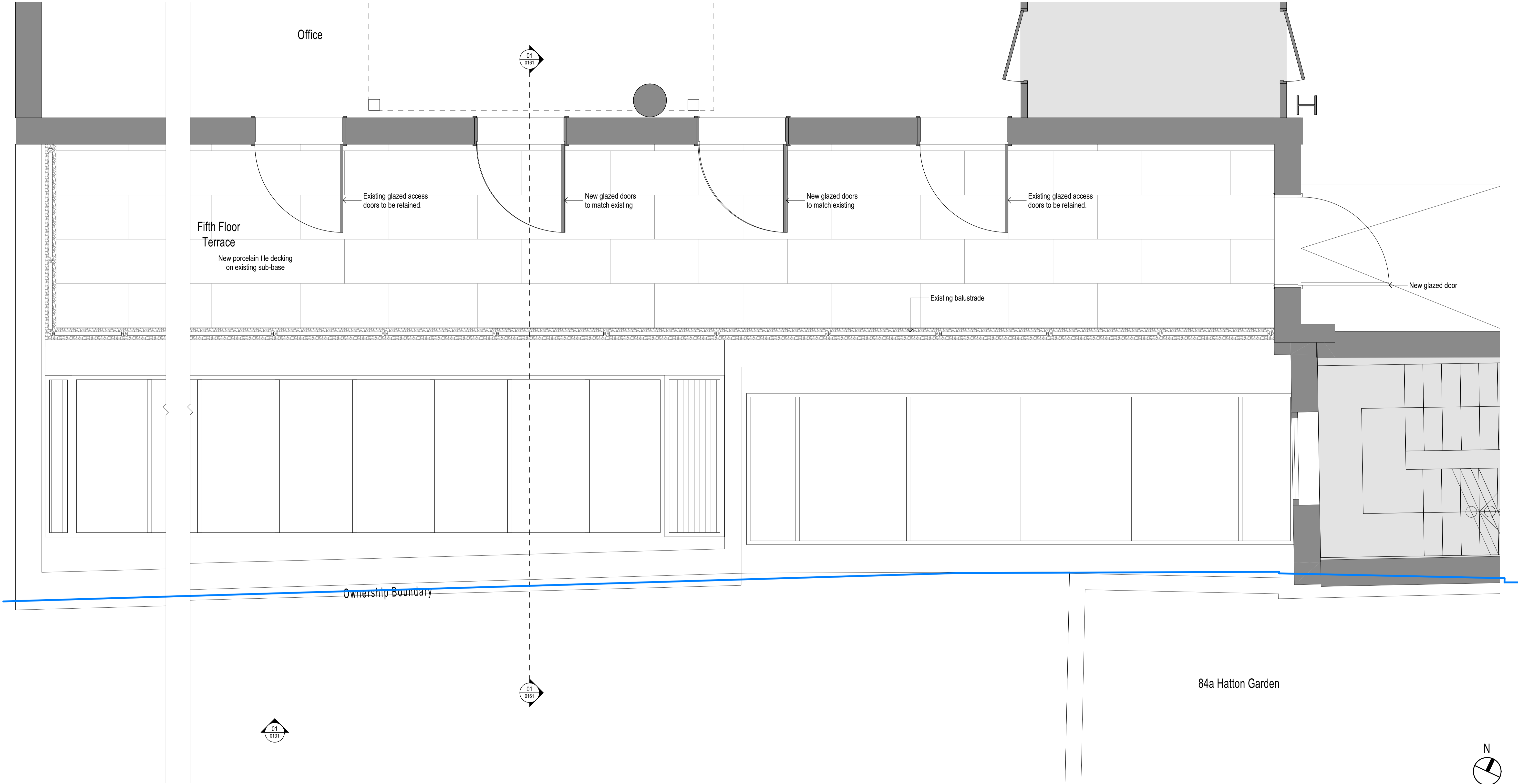
1 Proposed Fifth Floor Terrace Detail Plan SCALE 1:25
