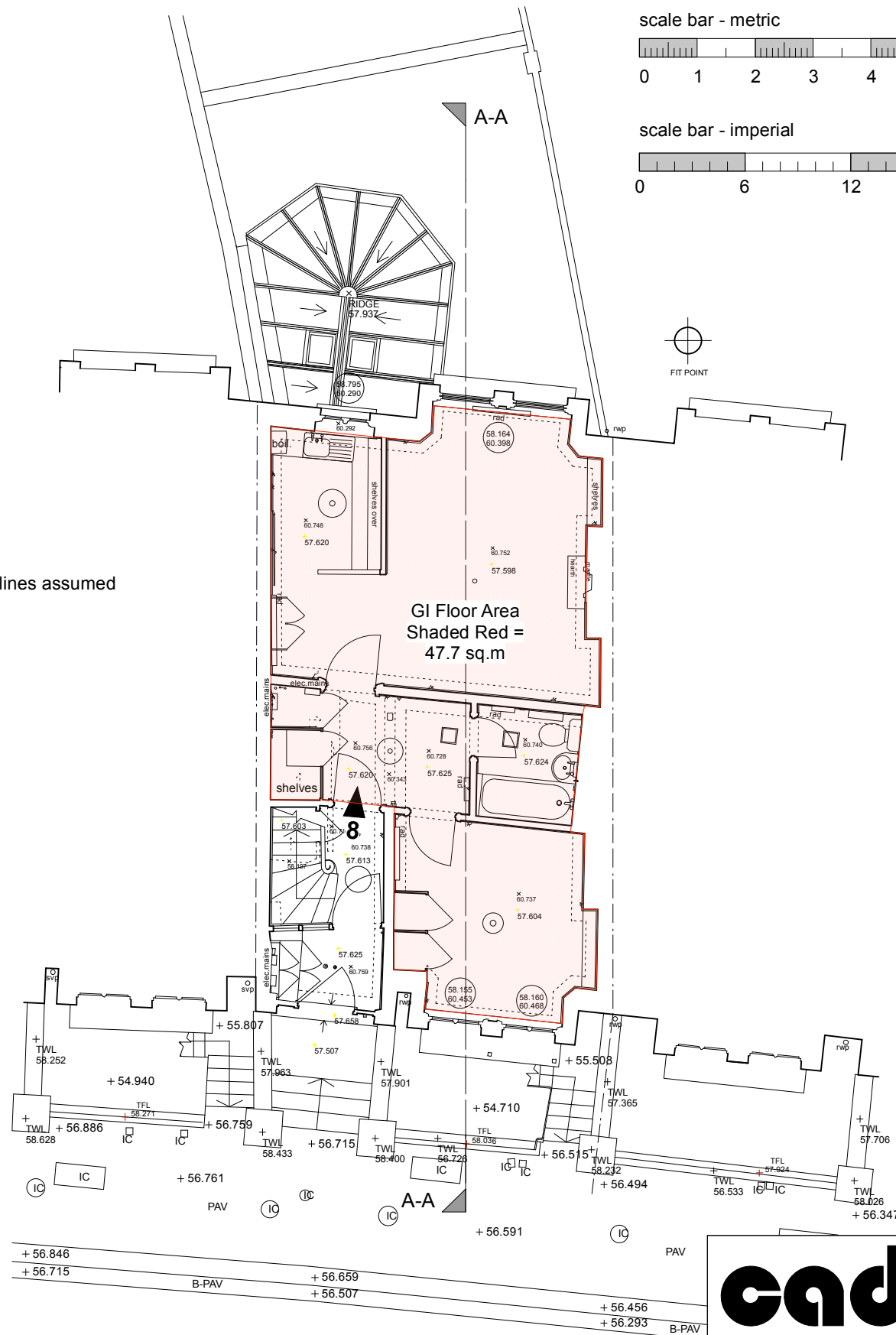
EXISTING UPPER GROUND FLOOR PLAN - No. 8
