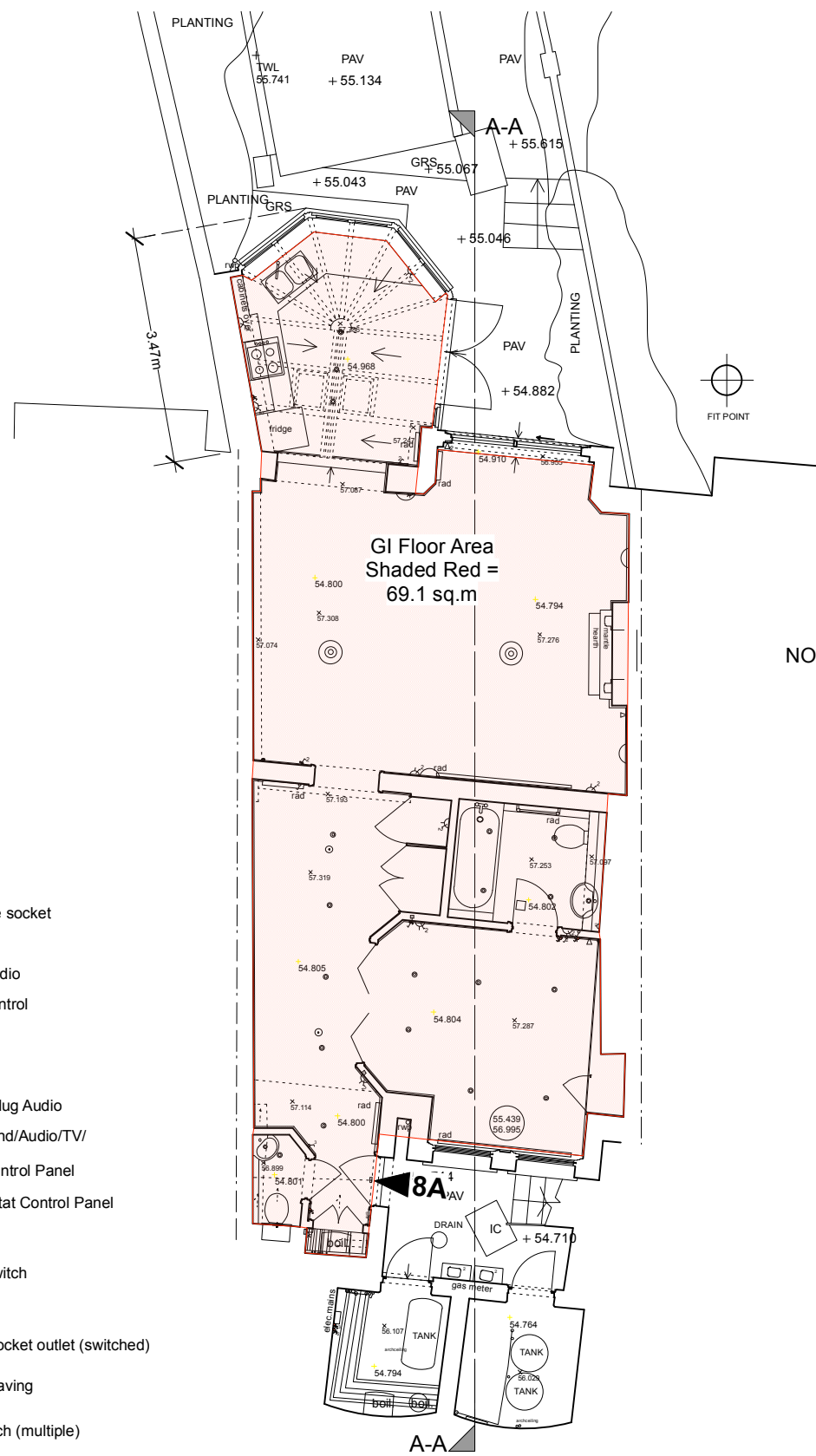
EXISTING LOWER GROUND FLOOR PLAN - No. 8A
