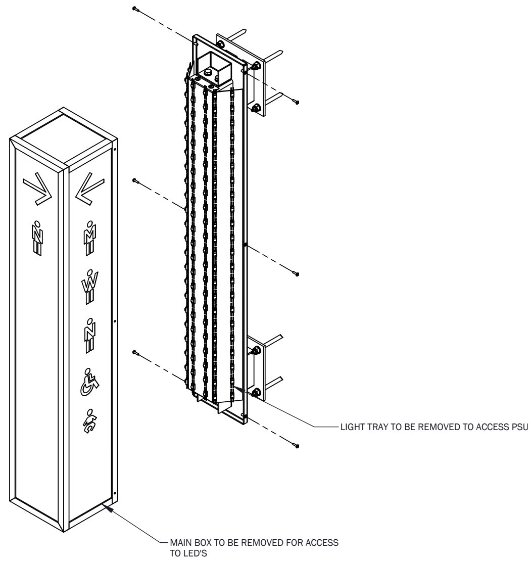
EXPLODED VIEW SCALE_1 : 10
