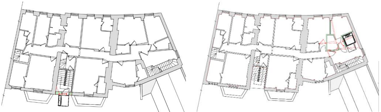
Figure 11. From left: External lift position (Option 1) on second floor indicating demolition (in red) and reconstruction (in green); Internal lift position to the southern end of the hotel (Option 2), adjacent to the stairwell of no.63. with associated demolition (in red) and reconstruction (in green).
