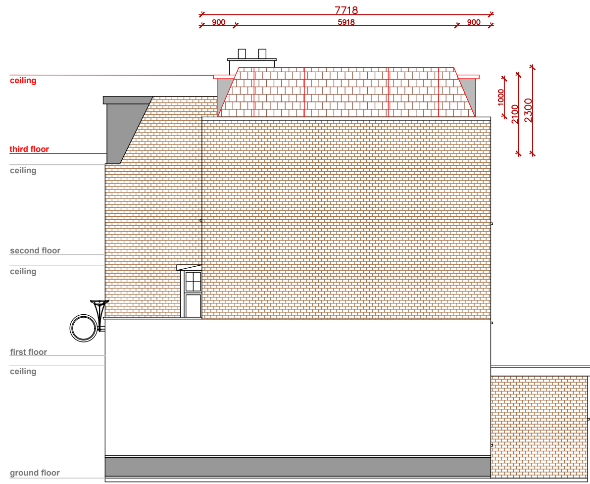
14 PROPOSED SIDE ELEVATION 1:100 @A3
