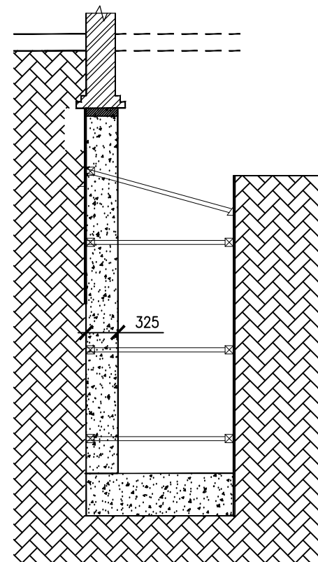
STAGE 5 - CONCRETE BASE OF PIN
