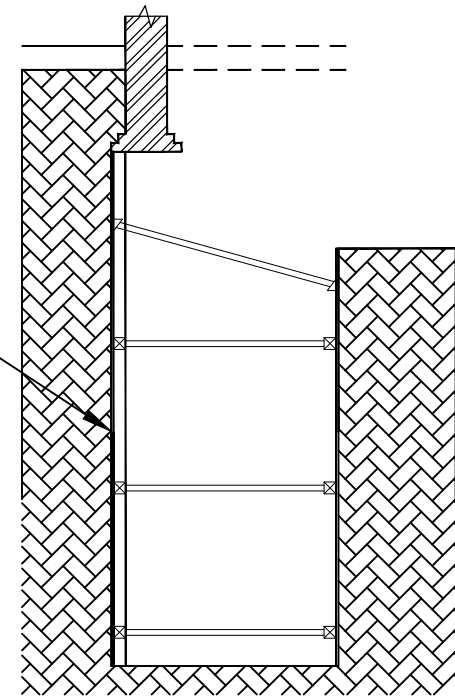
STAGE 3 - EXCAVATE FOR PIN
