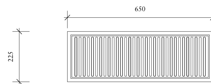
5 Cast Iron Grill detail - lintel level 1:10
