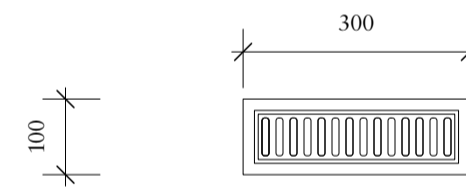
02 Cast Iron Grill detail - plinth level 1:10
