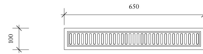
03 Cast Iron Grill detail - plinth level 1:10
