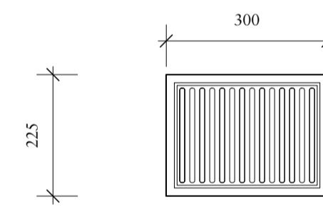
04 Cast Iron Grill detail - plinth level 1:10
