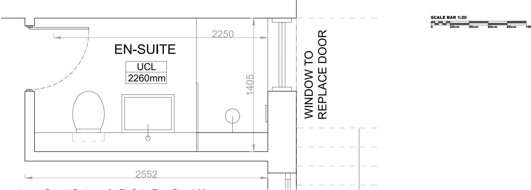
Lower Ground Bedroom 2 - En-Suite Floor Plan 1:20
