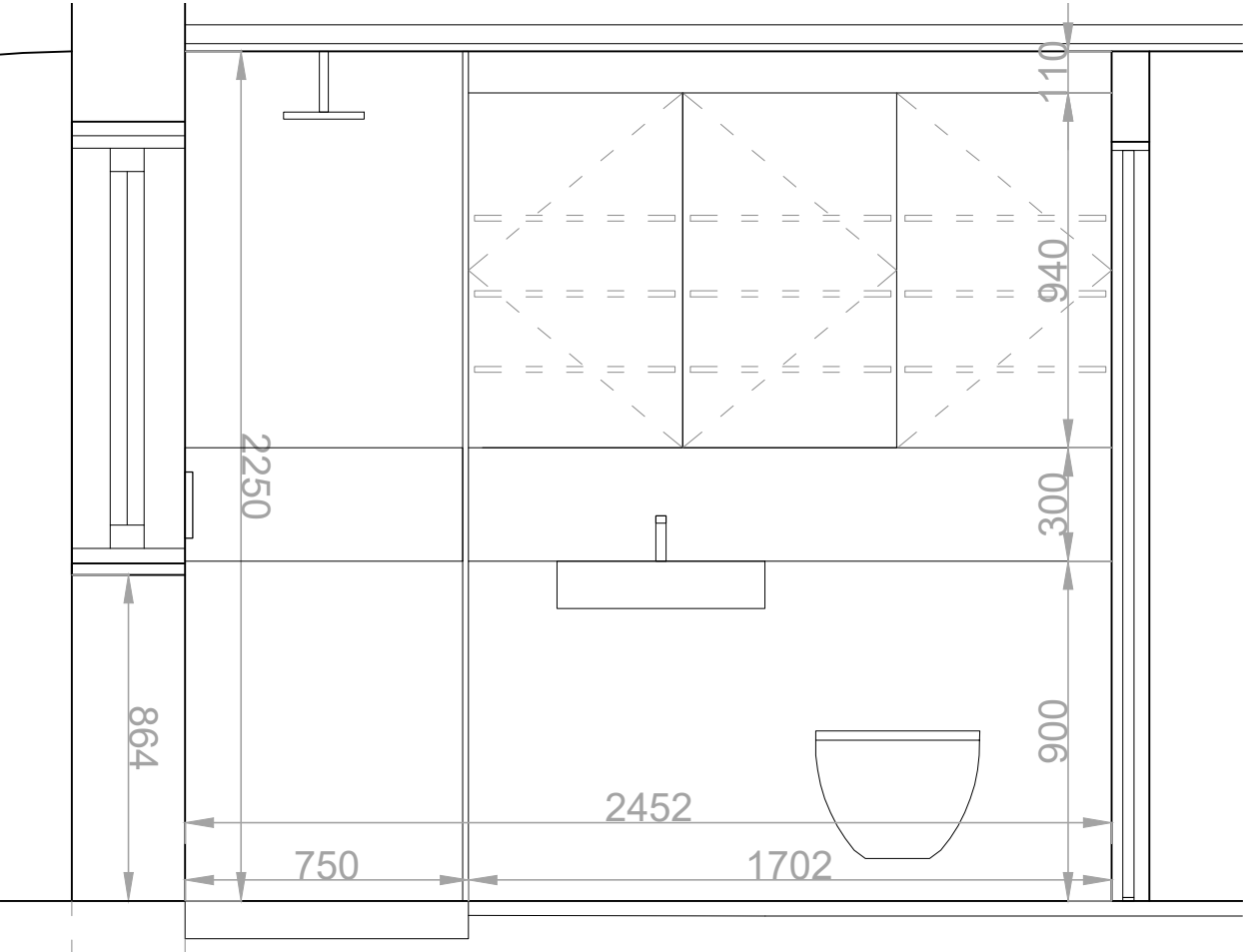
Lower Ground Bedroom 2 - En-Suite Elevation 3 - 1:20
