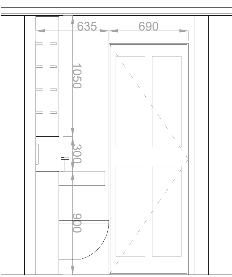
Lower Ground Bedroom 2 - En-Suite Elevation 2 - 1:20
