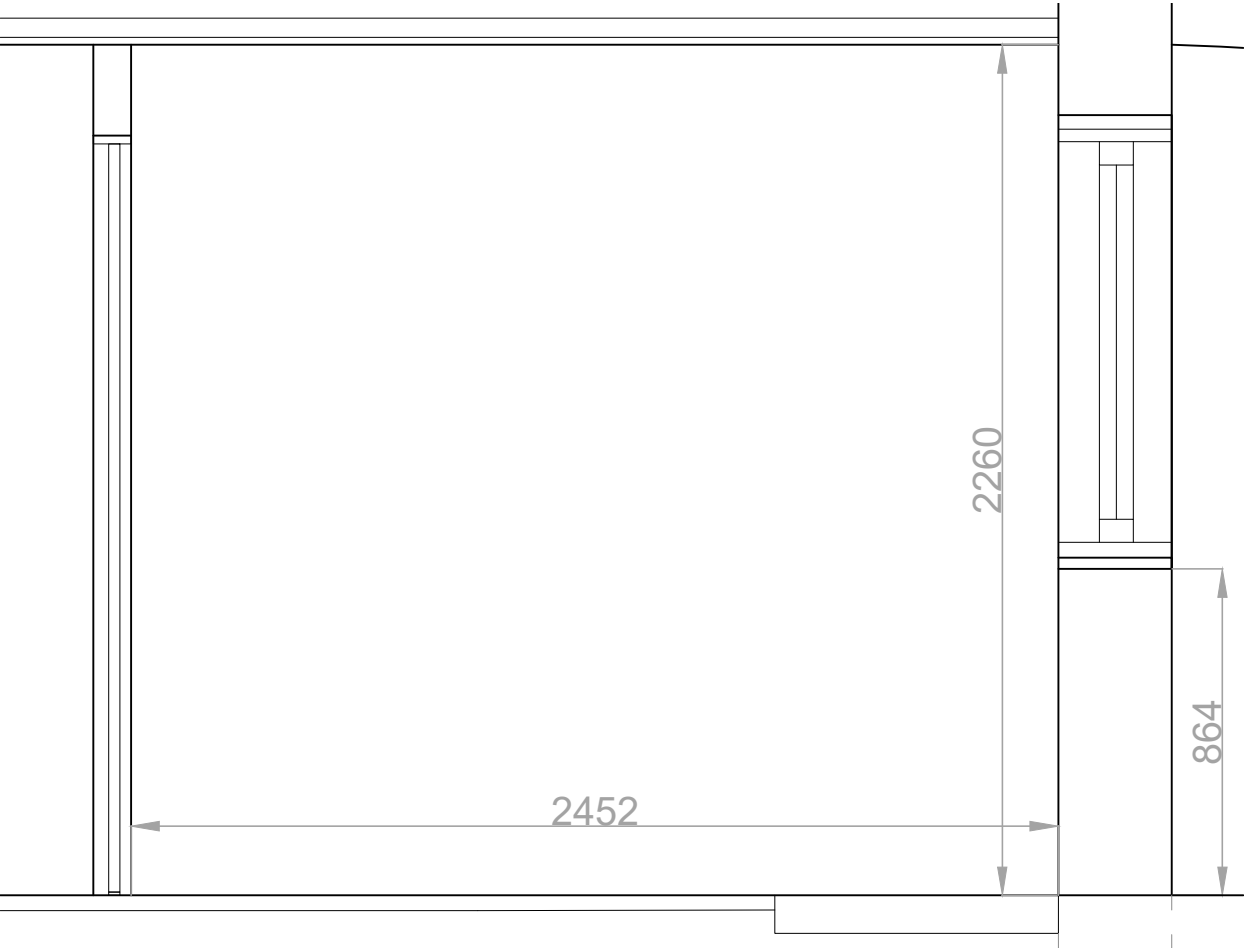
Lower Ground Bedroom 2 - En-Suite Elevation 1 - 1:20
