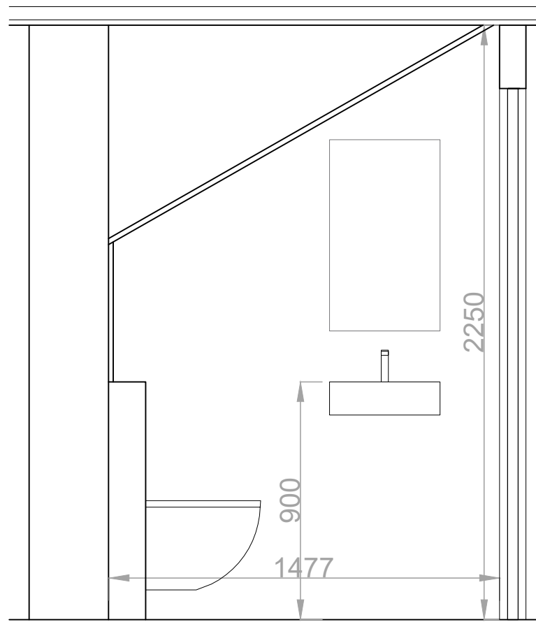
Lower Ground WC - Elevation 4 - 1:20
