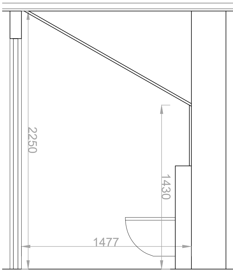
Lower Ground WC - Elevation 3 - 1:20
