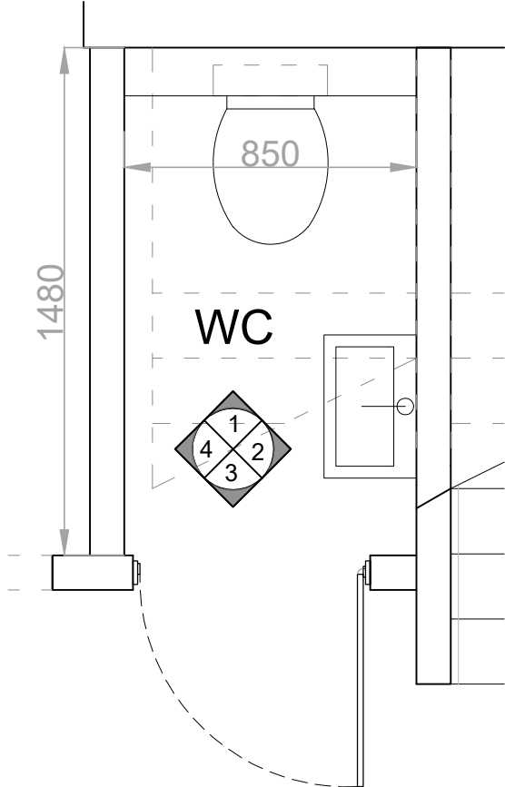
Lower Ground WC - Floor Plan 1:20
