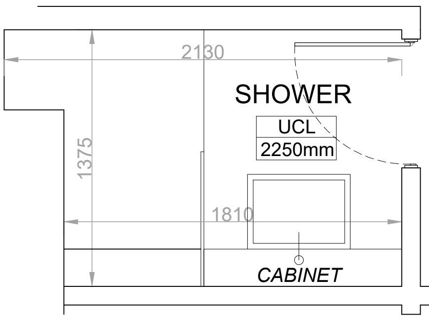
Lower Ground Bedroom 1 - Shower Floor Plan 1:20
