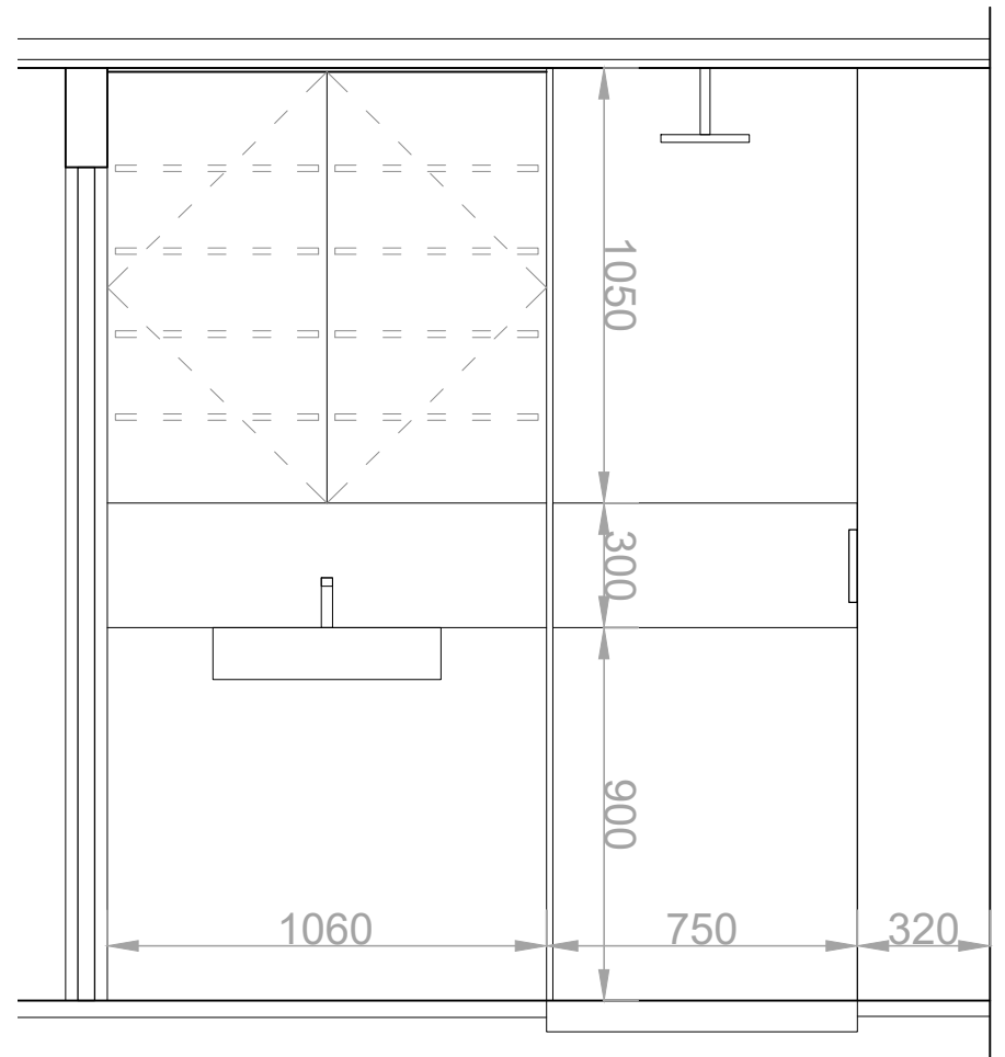
Lower Ground Bedroom 1 - Shower Elevation 2 - 1:20
