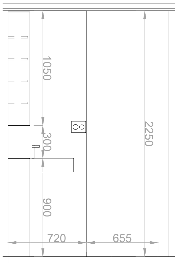
Lower Ground Bedroom 1 - Shower Elevation 3- 1:20
