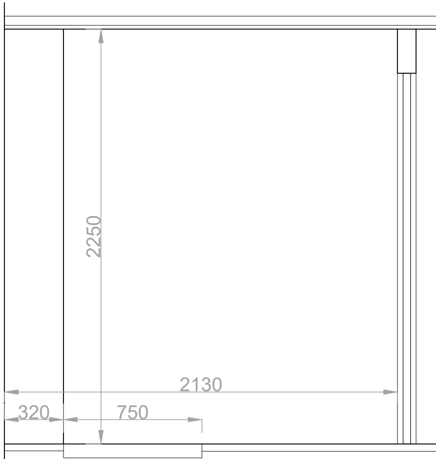
Lower Ground Bedroom 1 - Shower Elevation 1 - 1:20
