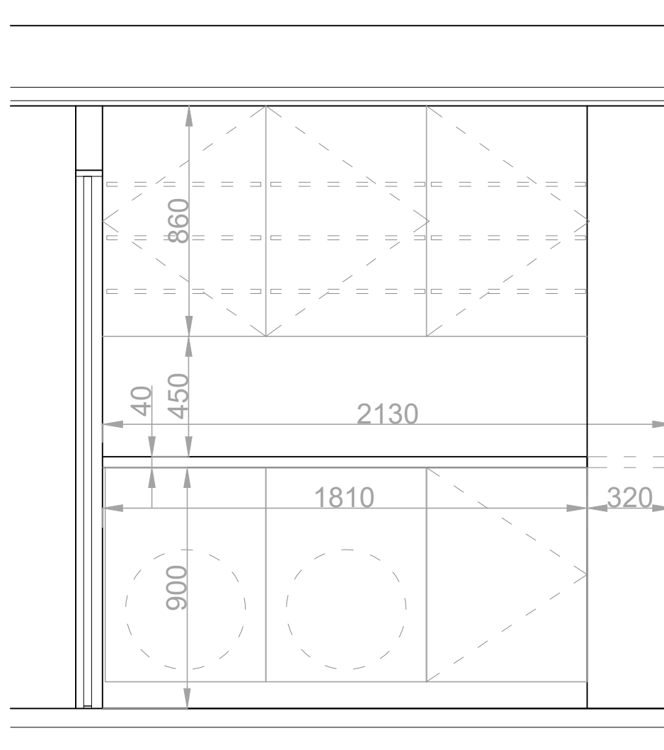
Utility Room Elevation 1:20
