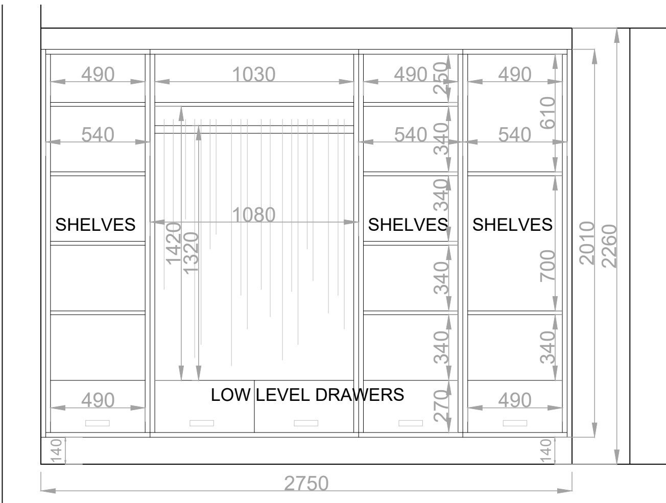
Lower Ground Bedroom 1 - Wardrobe (Open) Elevation 1:20
