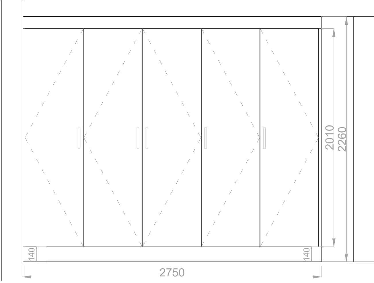
Lower Ground Bedroom 1 - Wardrobe Elevation 1:20
