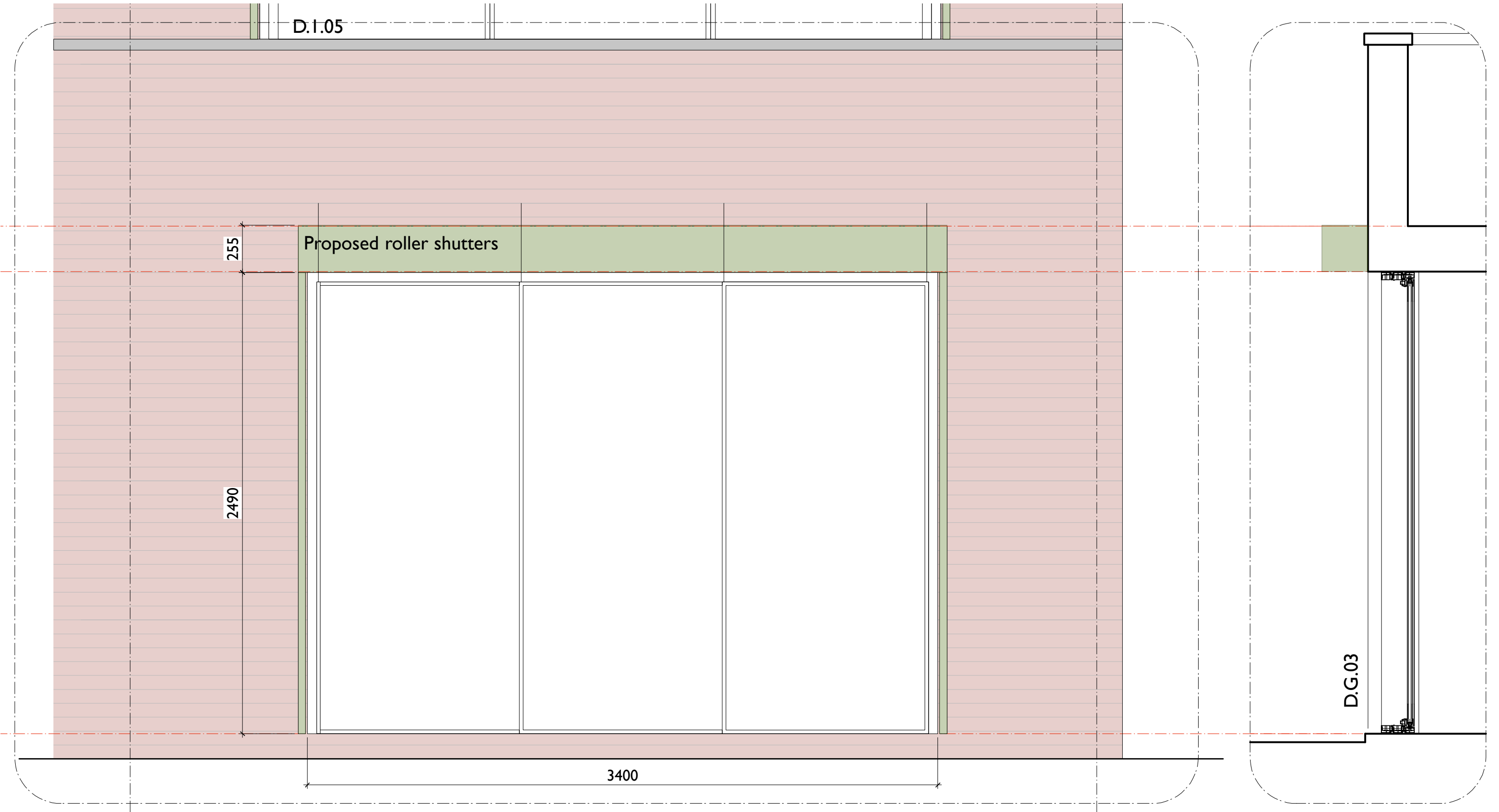
REAR ELEVATION
