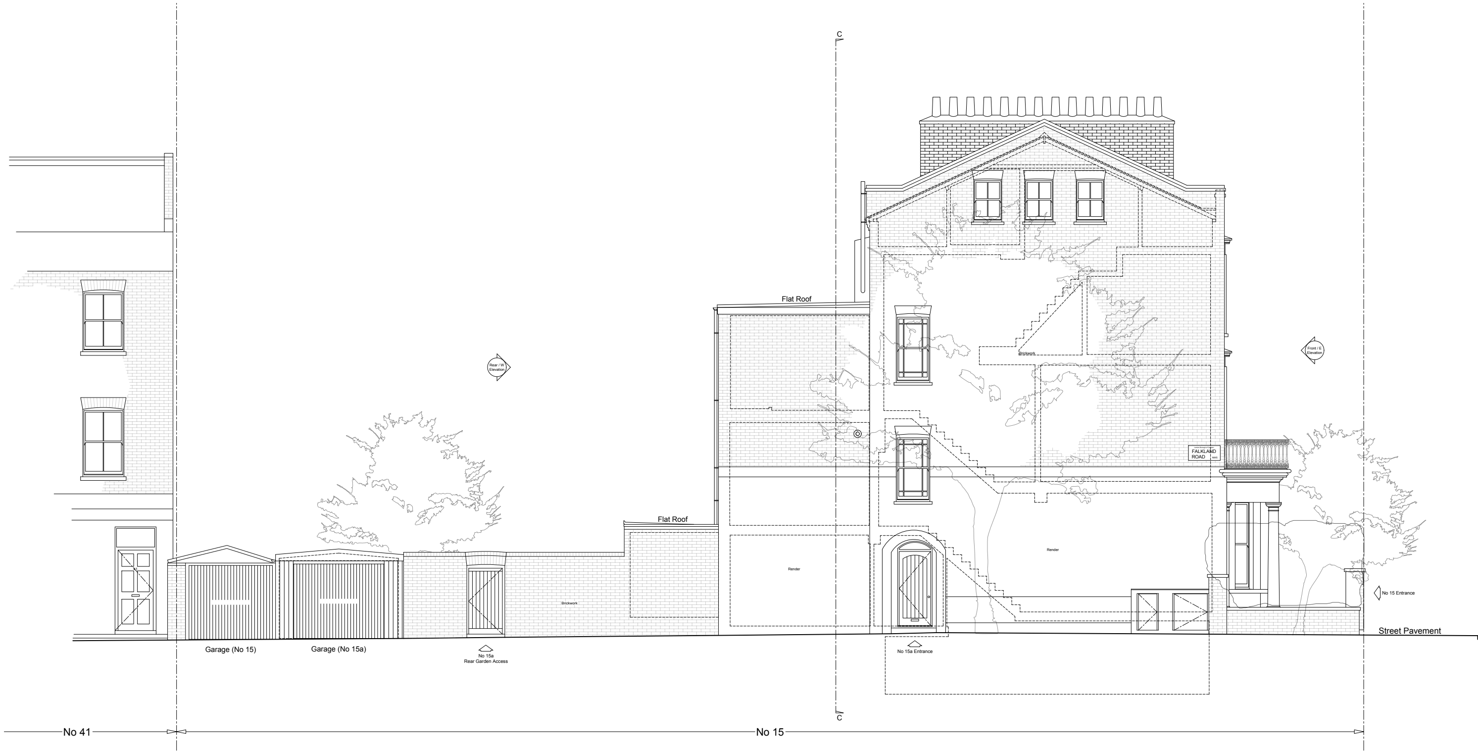
EXISTING SIDE ELEVATION 1:100
