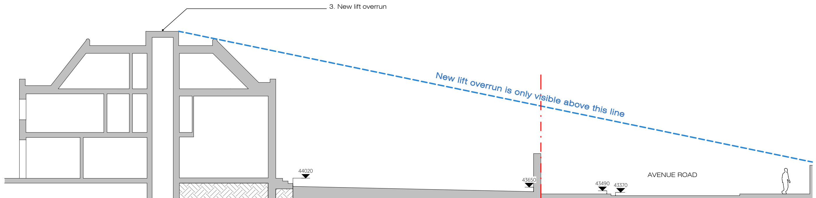
SECTION E - THROUGH LIFT OVERRUN
