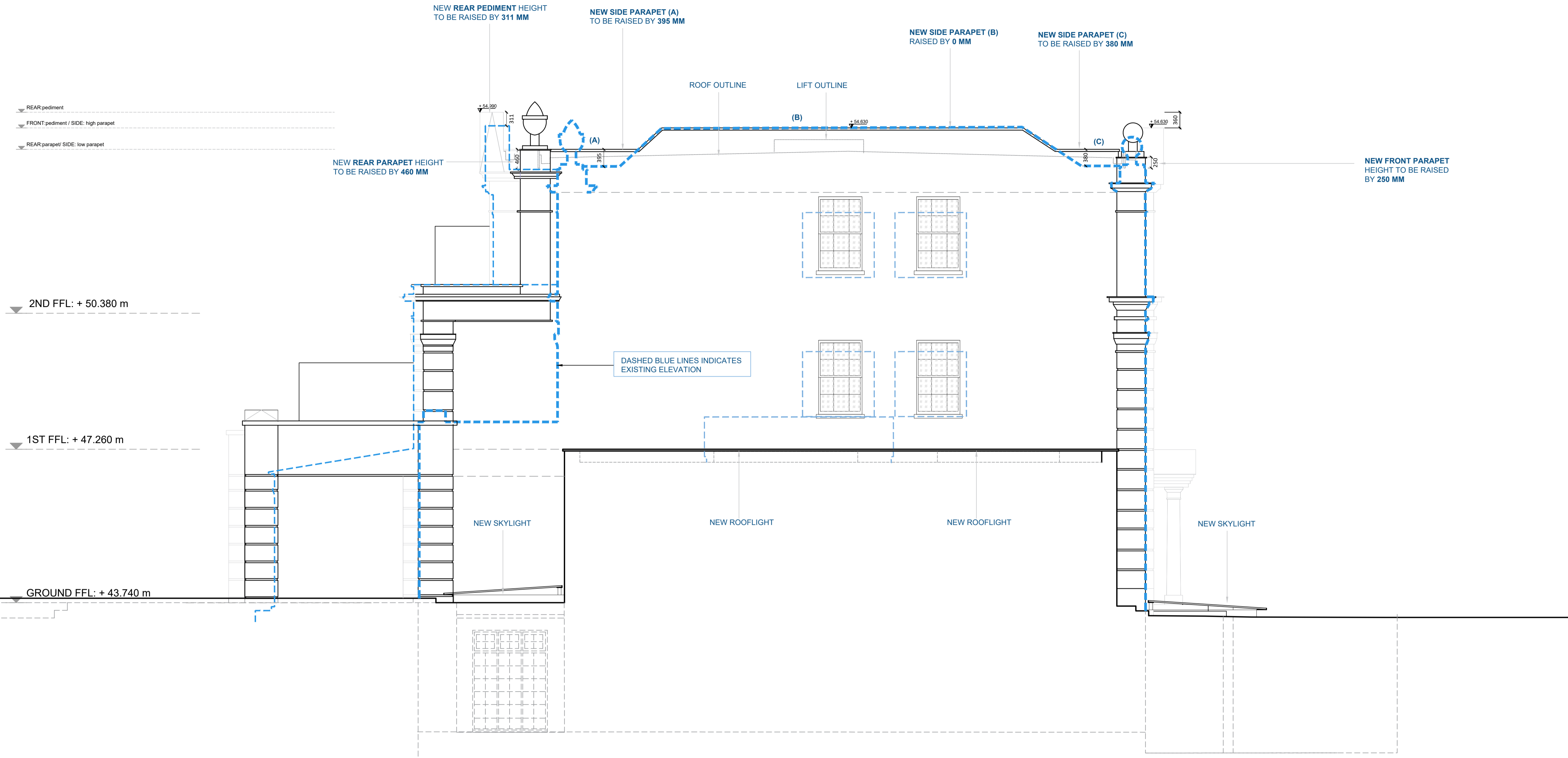
04 PROPOSED - ELEVATION 4 - SIDE SCALE 1:50 @ A1
