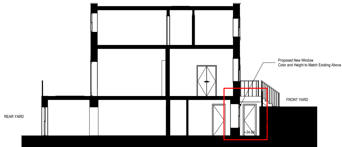
2 Proposed Section 1 : 100
