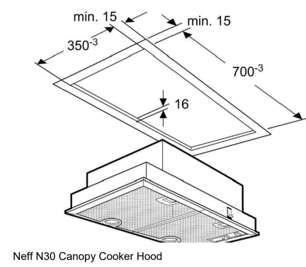
Neff N30 Canopy Cooker Hood
