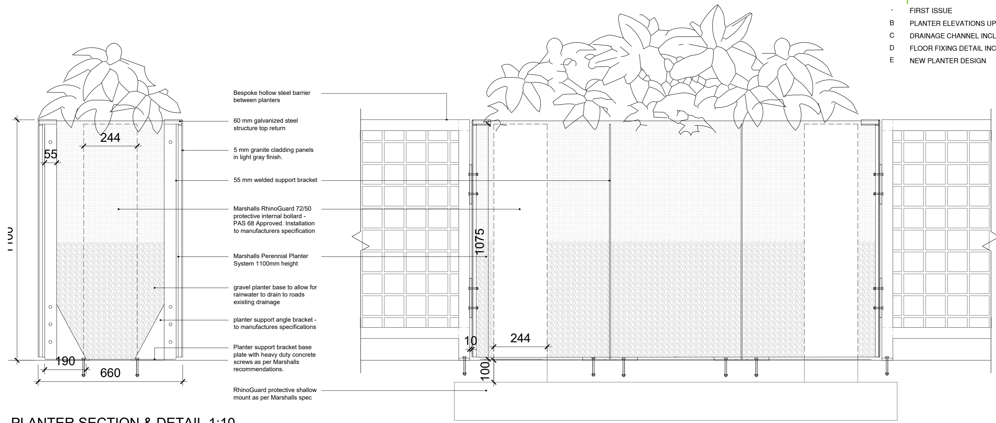
PLANTER SECTION & DETAIL 1:10
