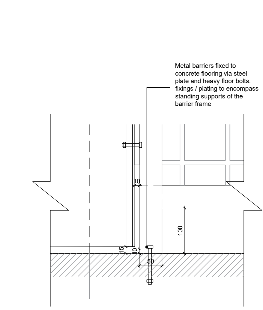
PLANTER FIXING DETAILS 1:5
