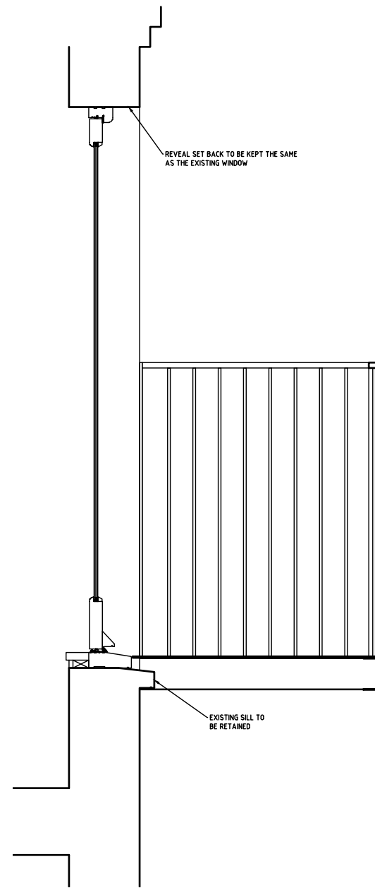
1:20 SECTIONAL DETAIL
