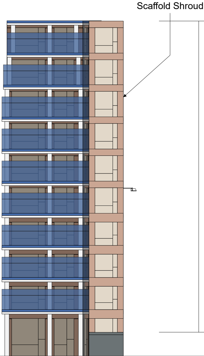
EAST ELEVATION
