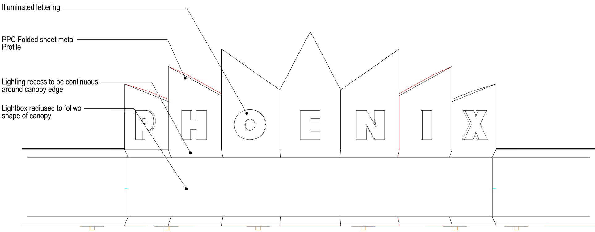
2 DETAIL Front Elevation of Corner 1:20
