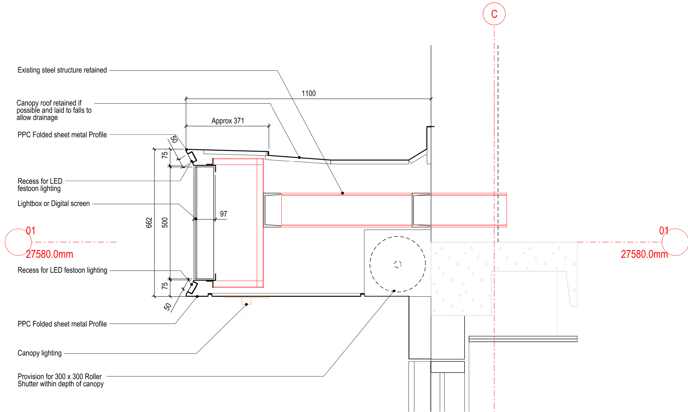
1 DETAIL Typical Section Thru Canopy 1:10
