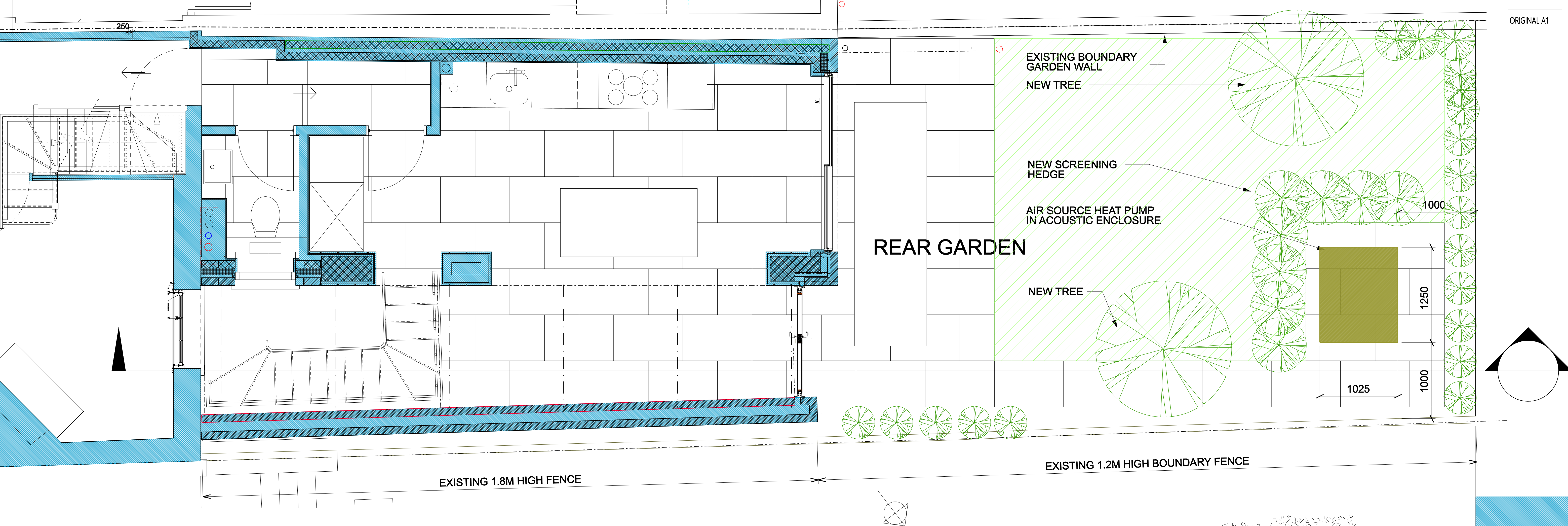
PART PLAN REAR EXTENSION AND GARDEN
