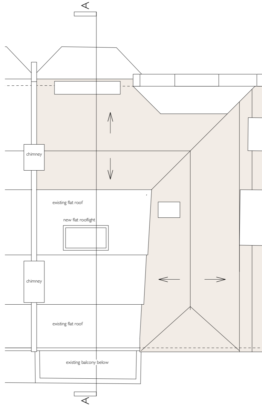
2 Proposed Roof Plan 1:100
