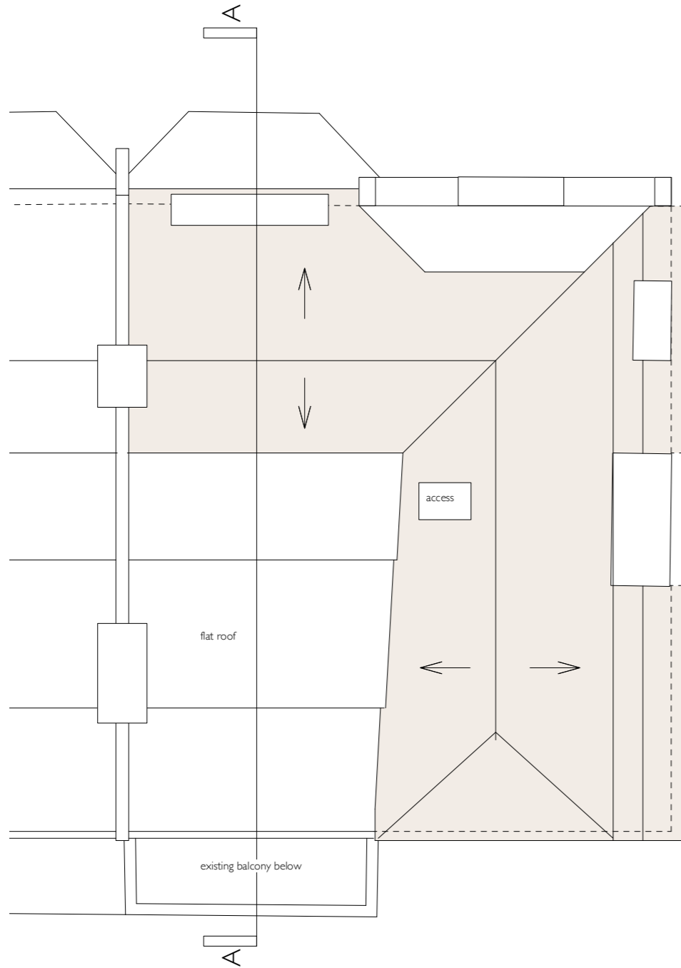
1 Proposed Plan 1:100
