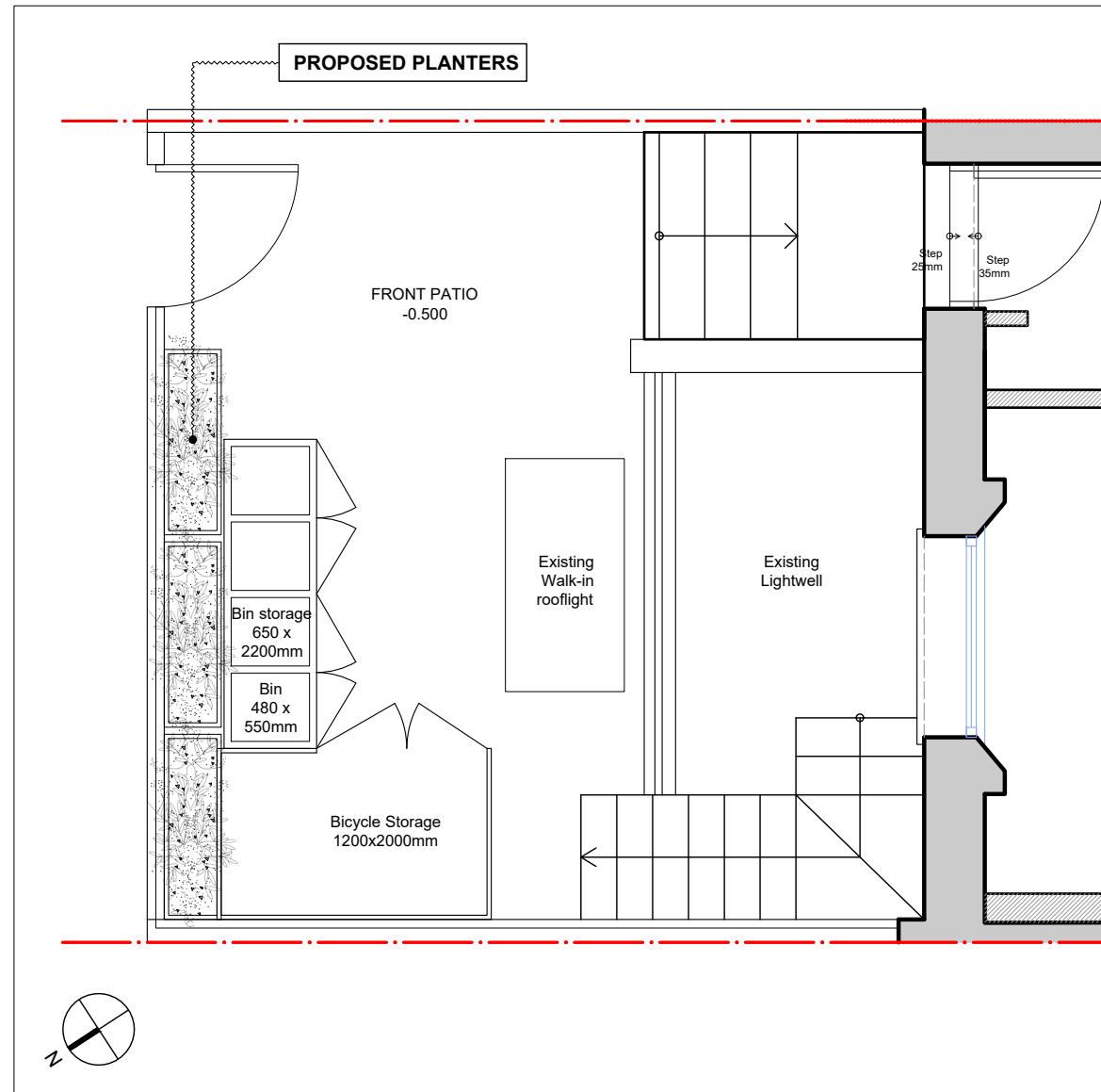
3 PROPOSED FRONT GARDEN PLAN
