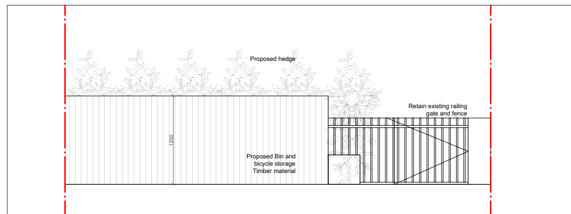
4 PROPOSED ELEVATION - INTERNAL VIEW
