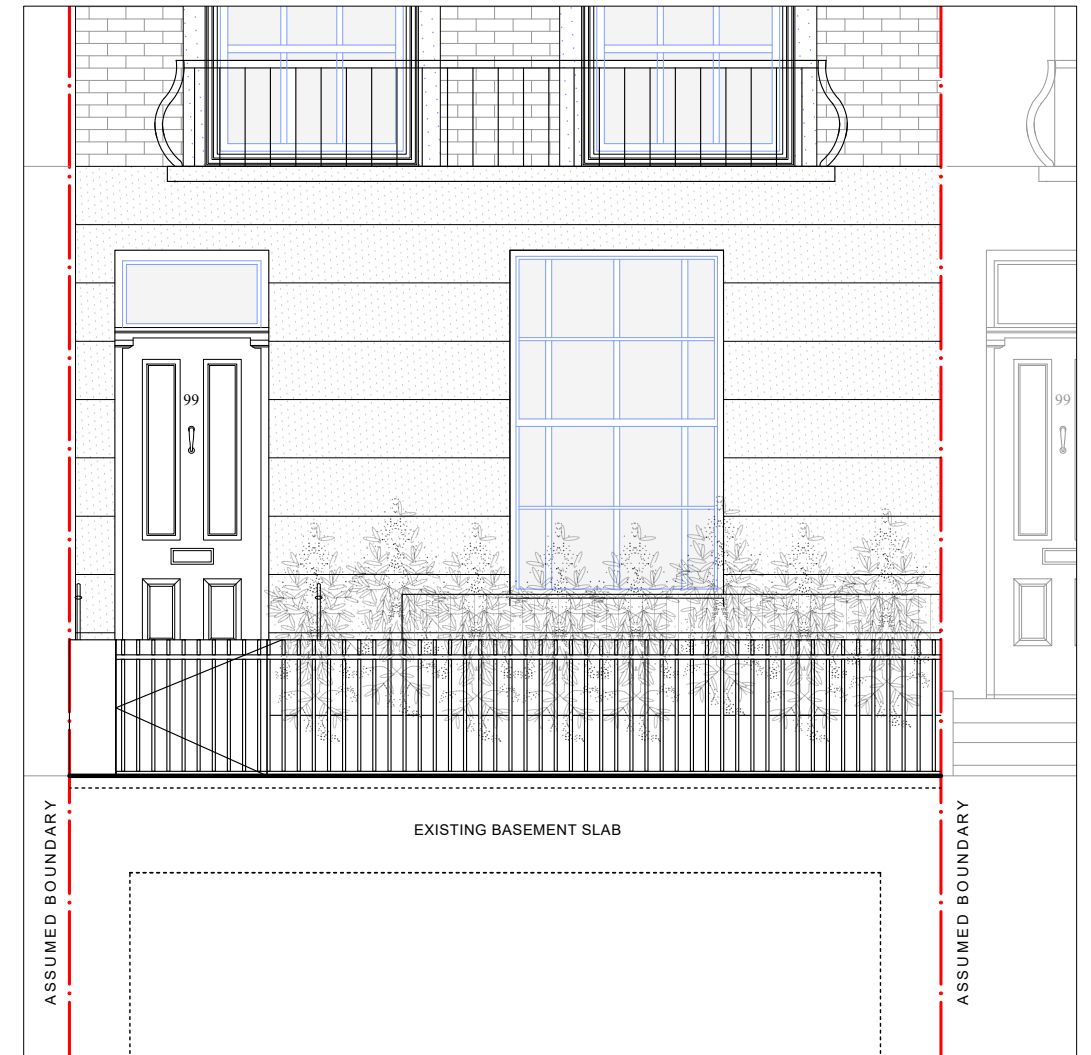
5 PROPOSED FRONT ELEVATION
