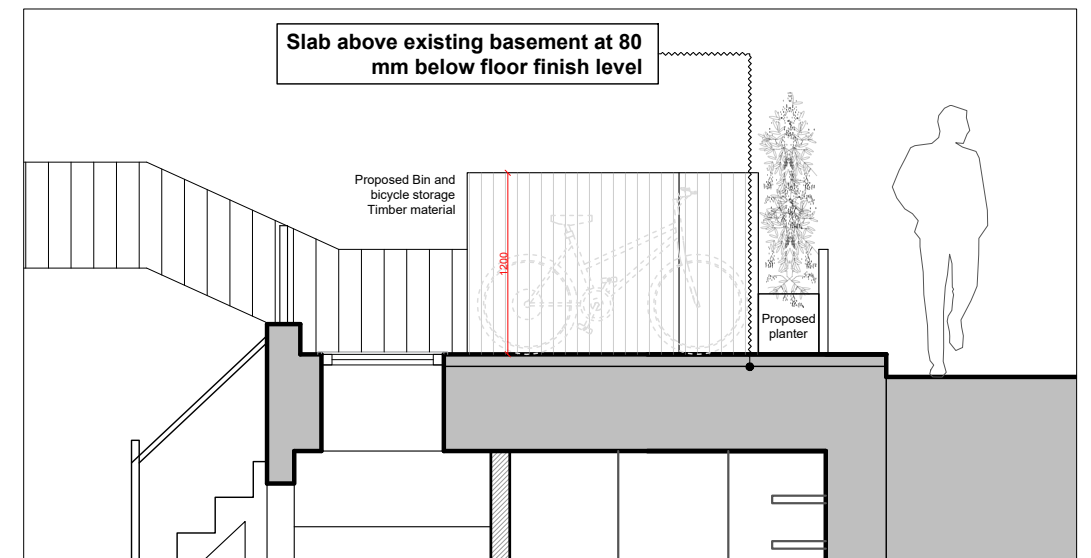
6 PROPOSED SIDE VIEW
