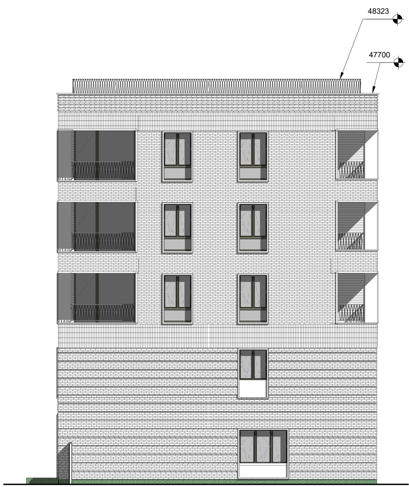
1 East Elevation (Courtyard) - Planning 1 : 100
