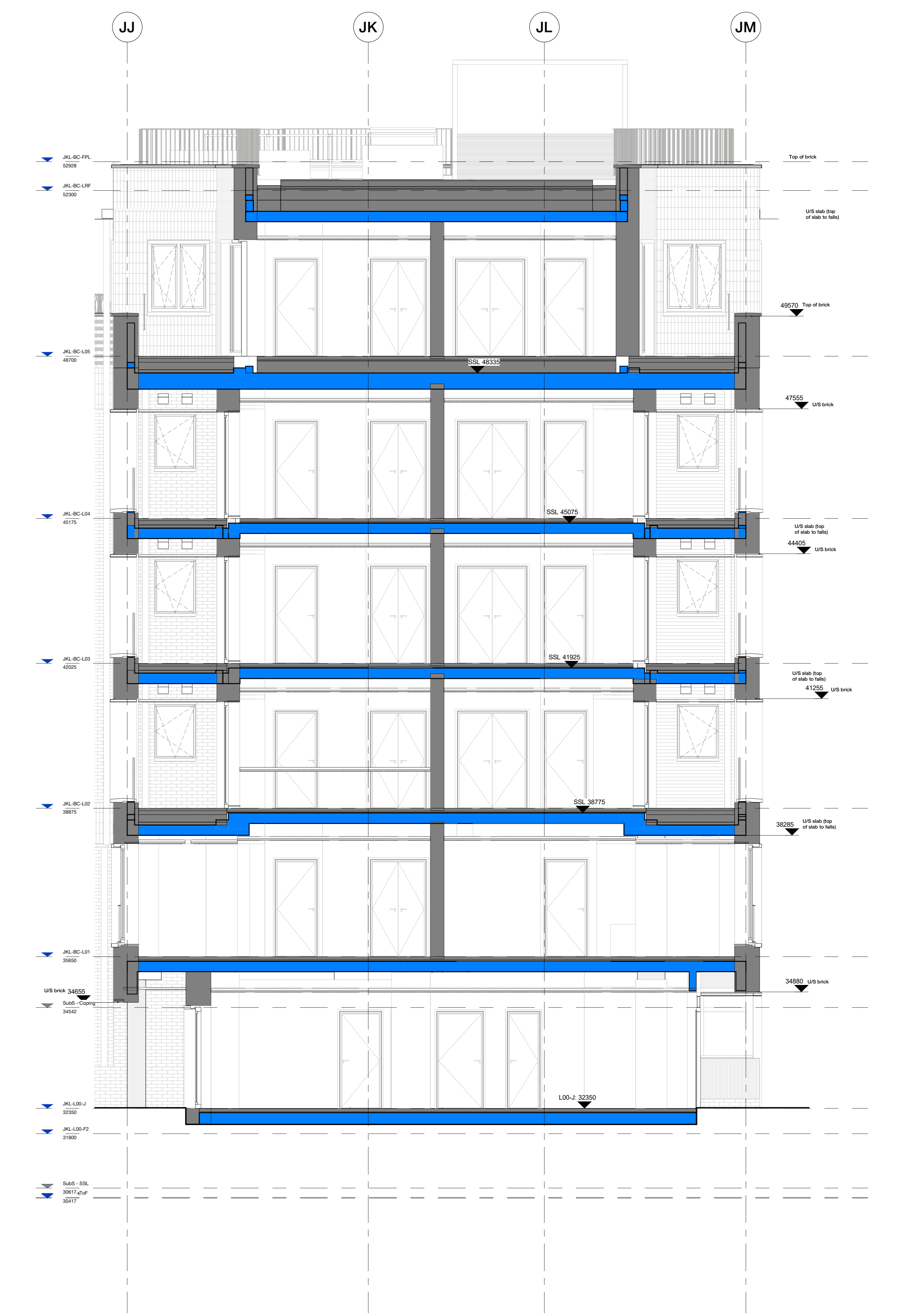
2 GA Sections - Cross Section D-D 1 : 50
