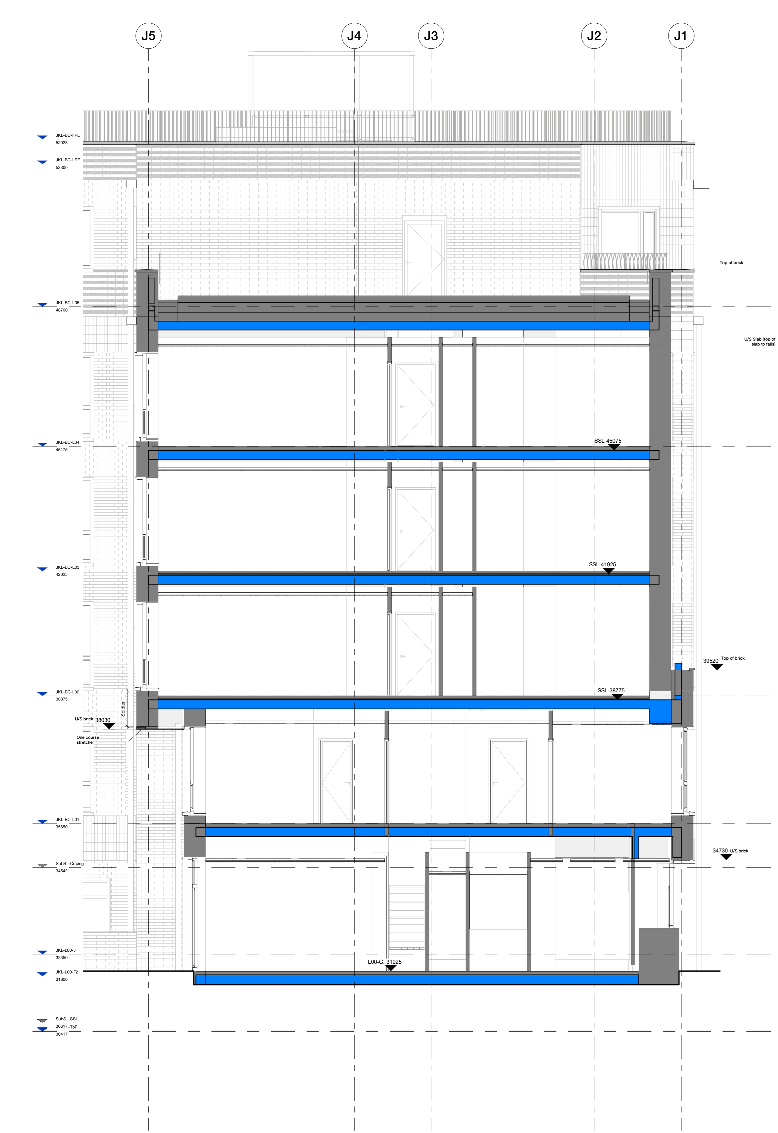
1 GA Sections - Cross Section C-C 1 : 50
