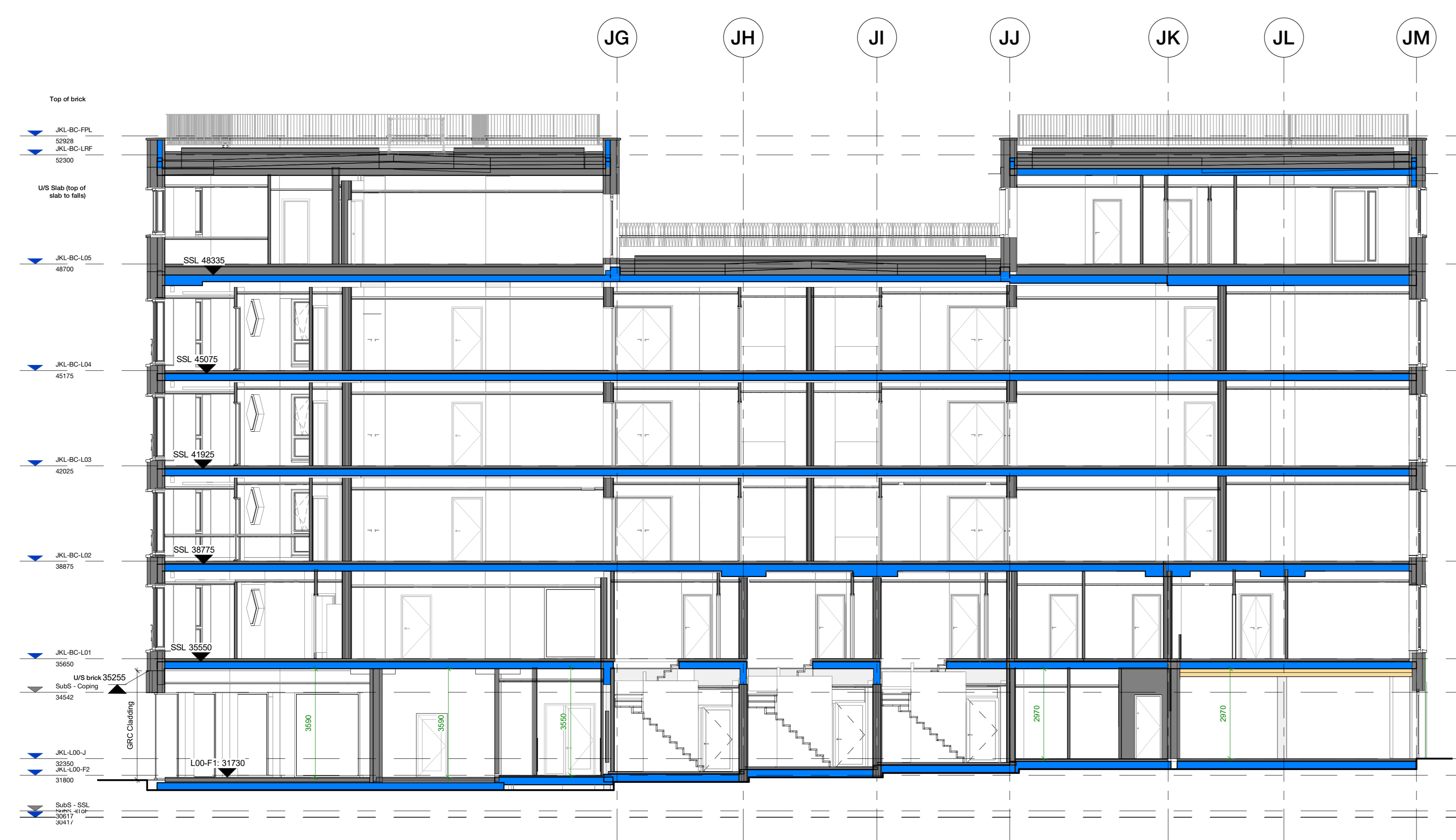
2 GA Sections - Long Section B-B 1 : 100
