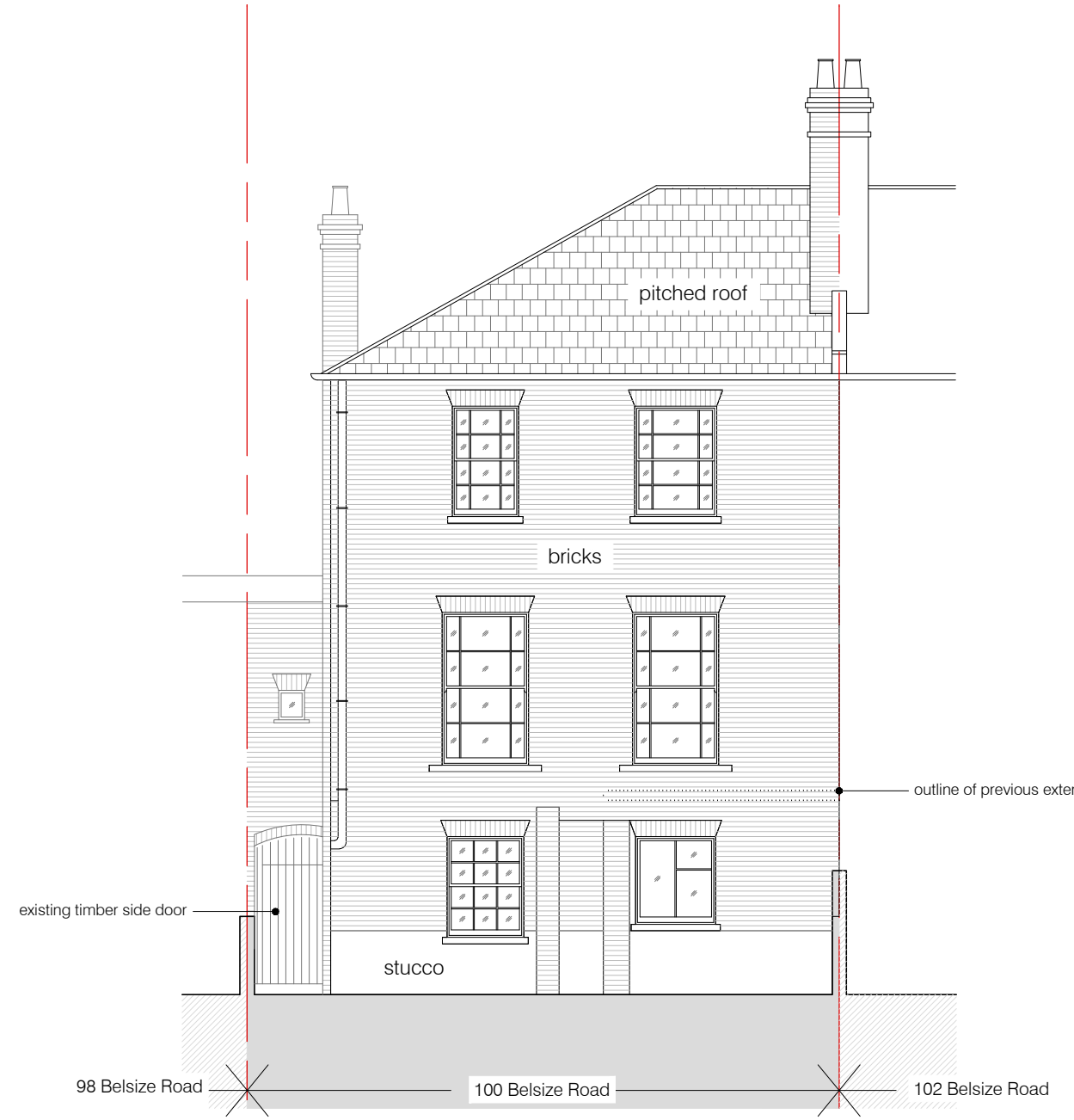
02 EXISTING REAR ELEVATION scale 1:100
