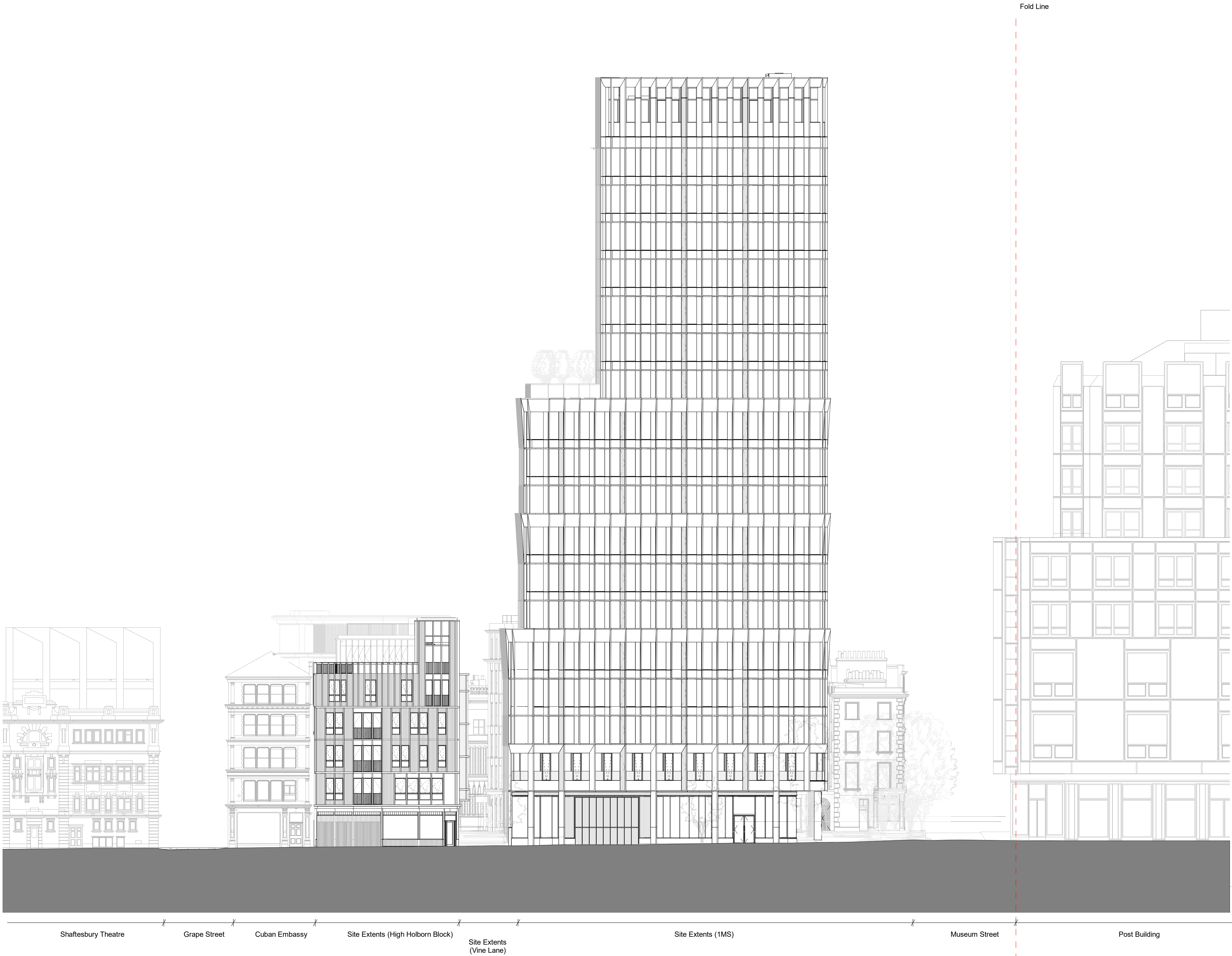
2 Proposed High Holborn Elevation 1 : 200
