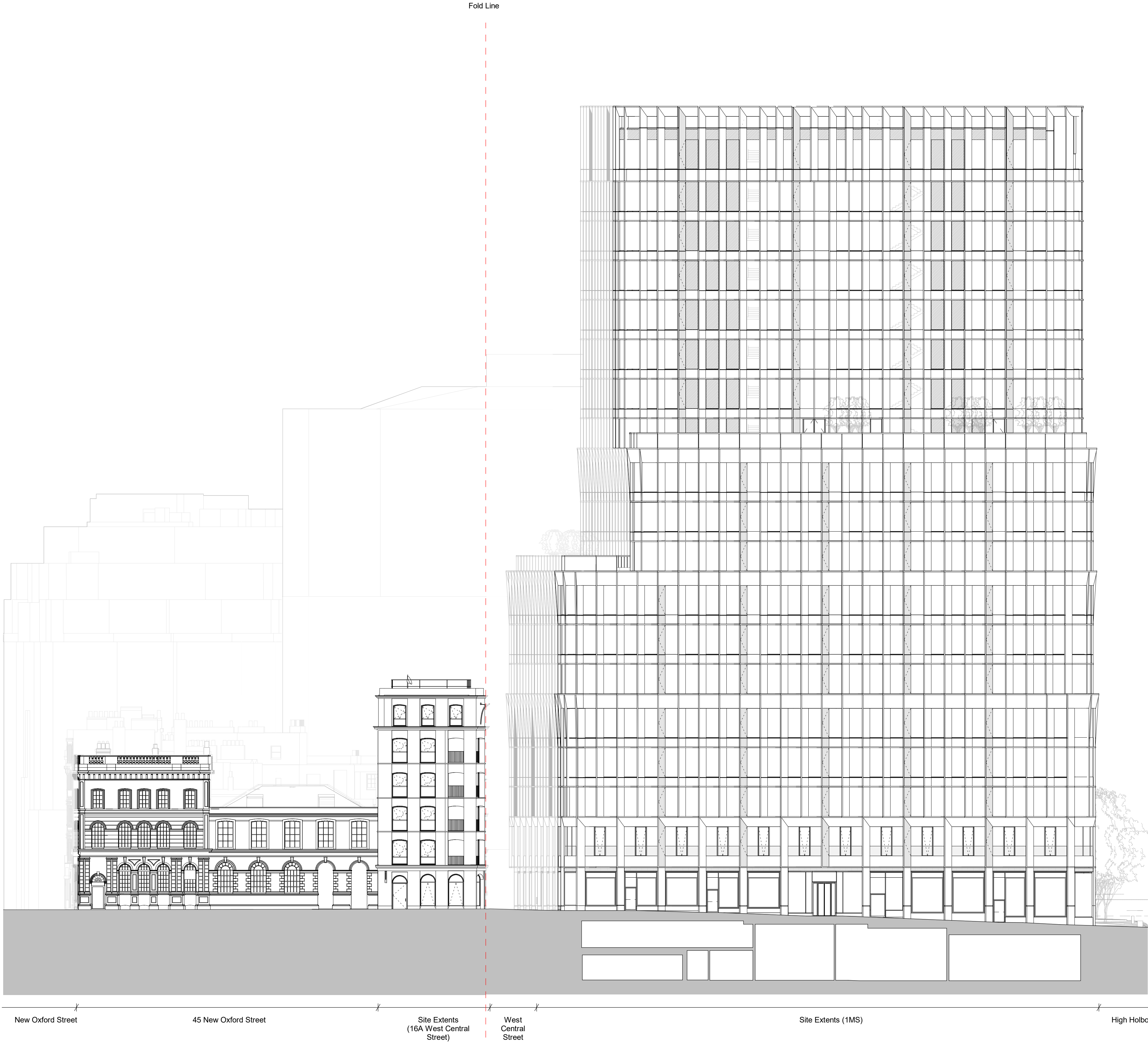
2 Proposed West Central Street Elevation - East
