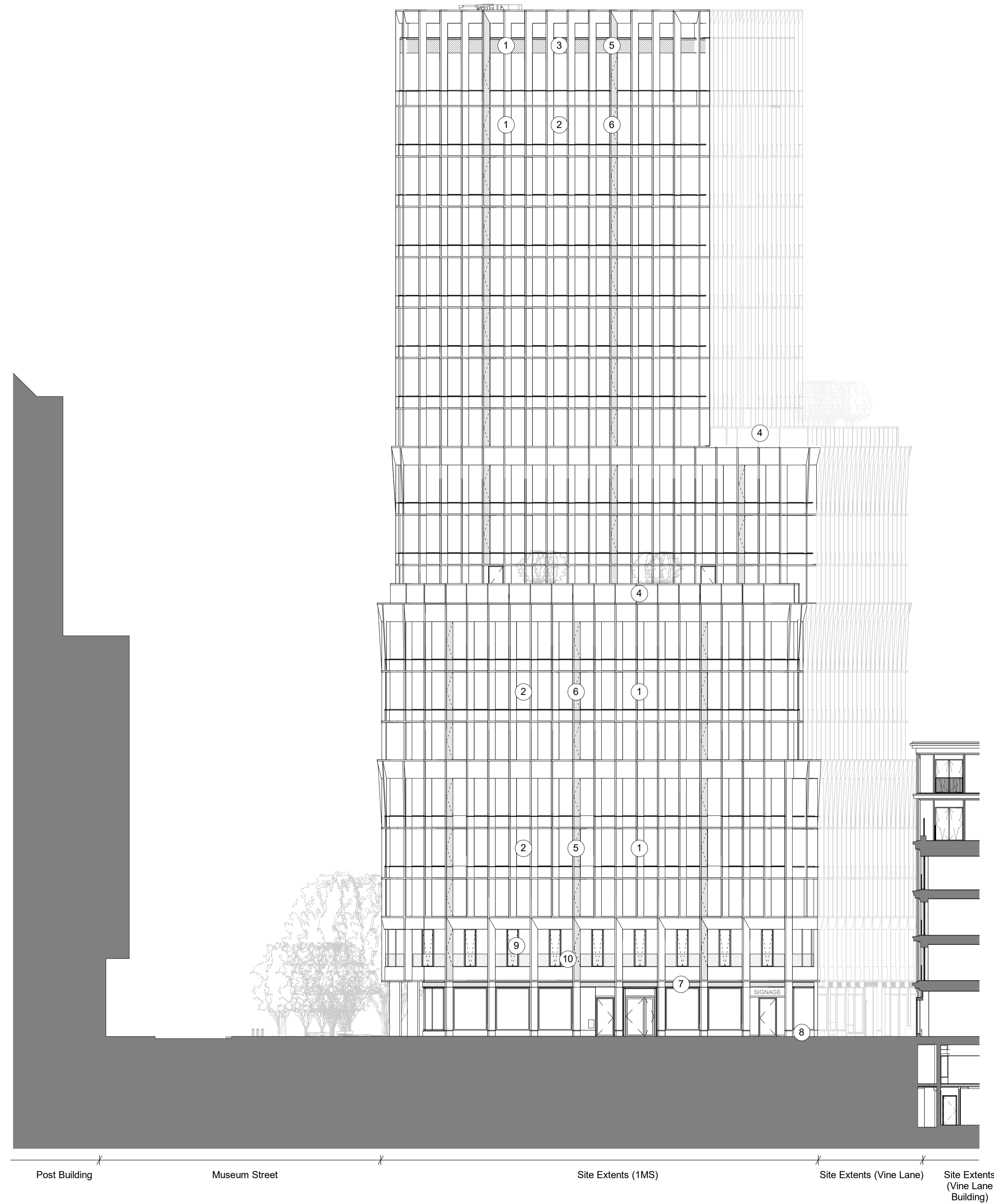
1 Proposed West Central Street Elevation (South) 1:200
