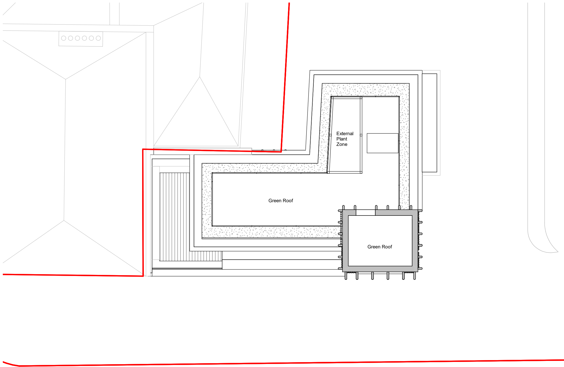
1 High Holborn Building - Proposed Roof Plan 1 : 100
