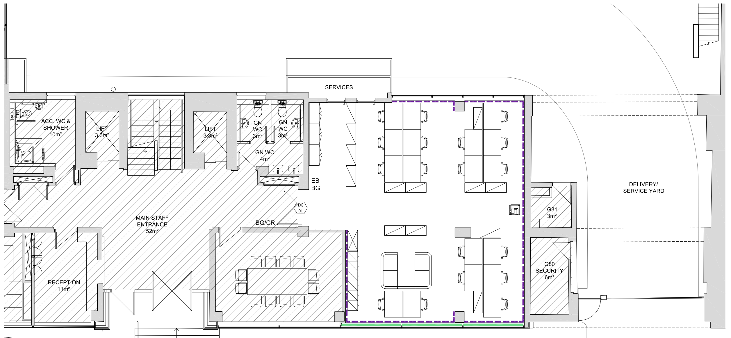
1 GROUND FLOOR PLAN AS EXISTING 1:50
