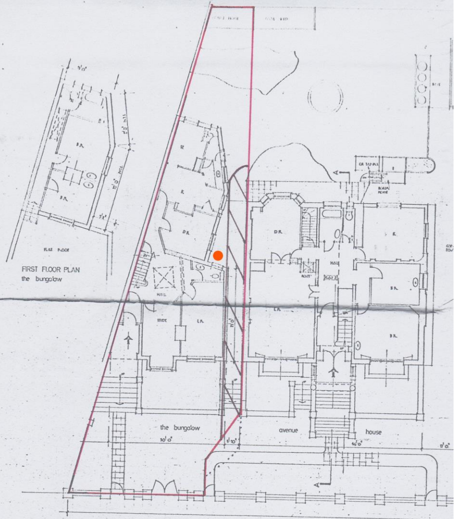
GROUND FLOOR PLANS and SITE PLAN
