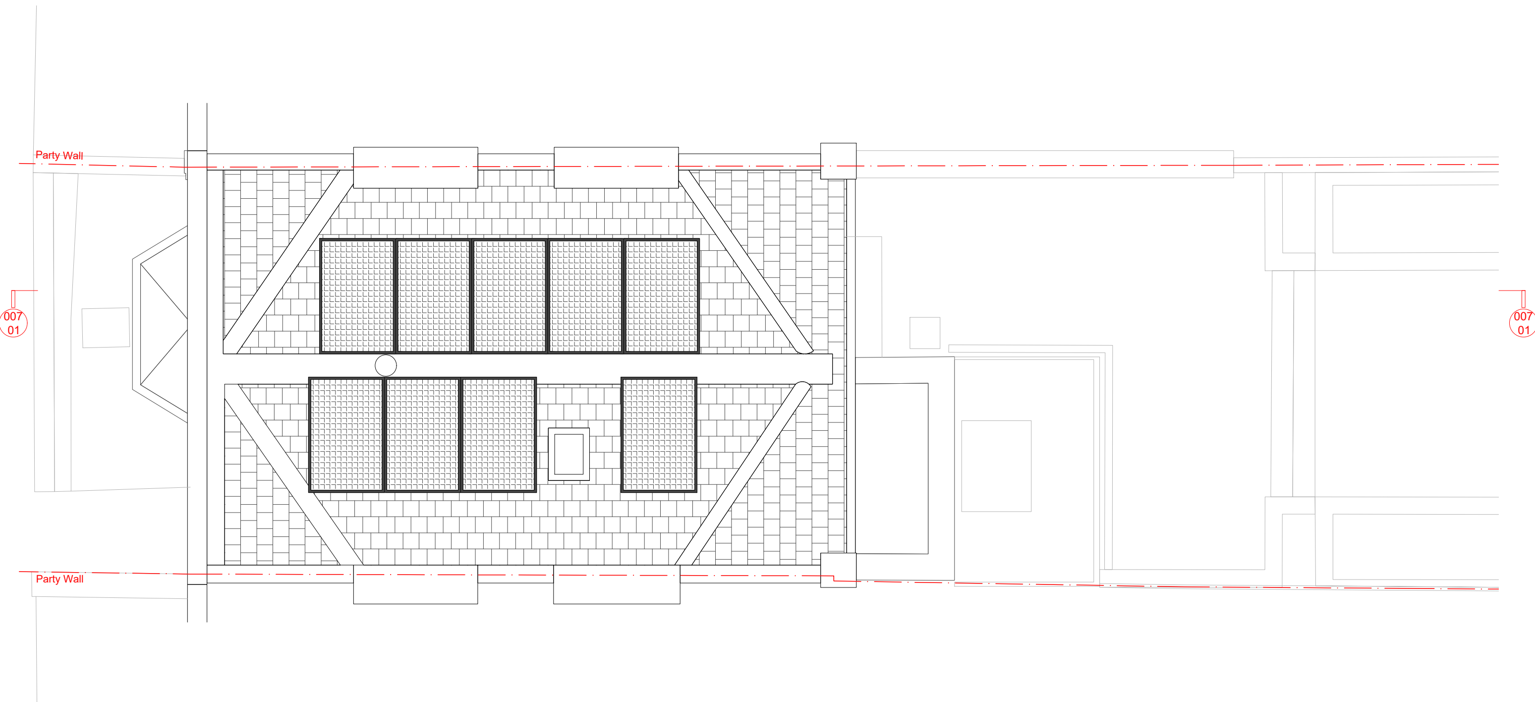
004 01 Existing Roof Plan Scale 1:50 @ A3 / 1:25 @ A1
