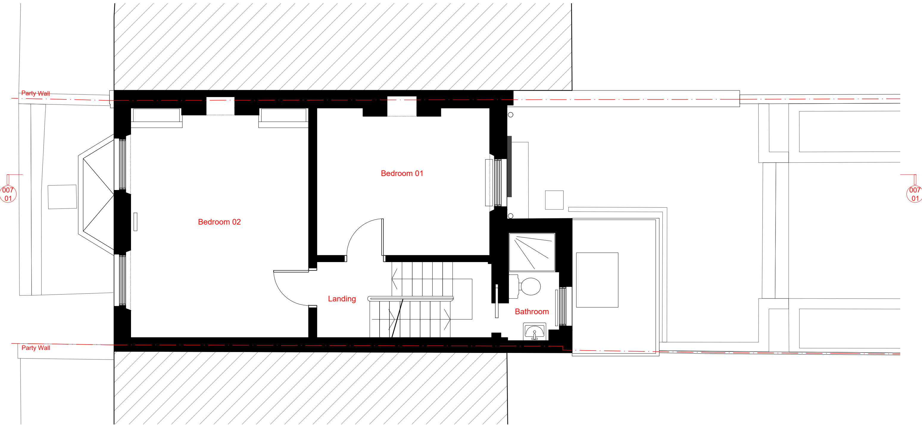
002 01 Existing 1st Floor Plan Scale 1:50 @ A3 / 1:25 @ A1
