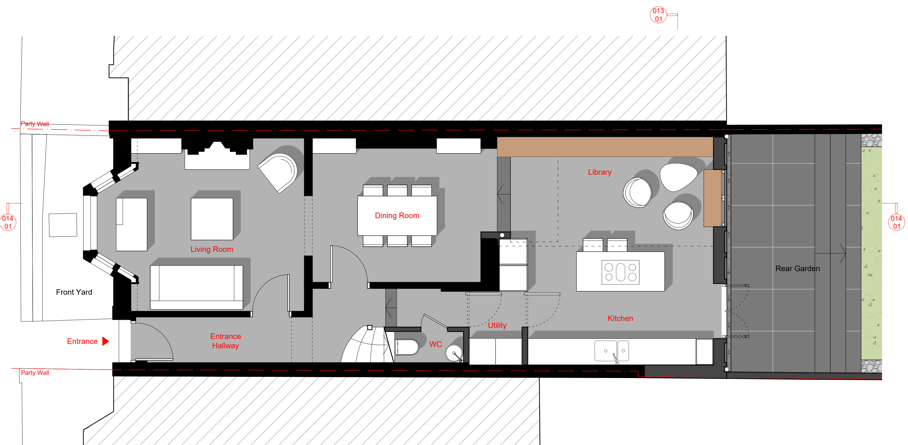
009 01 Proposed Ground Floor Scale 1:50 @ A3 / 1:25 @ A1
