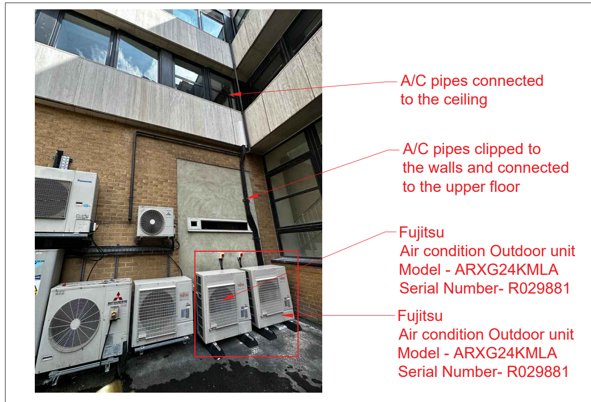
PROPOSED OUTDOOR A/C UNITS
