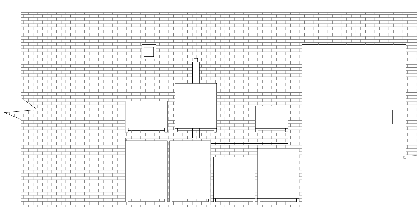
EXISTING REAR ELEVATION scale 1:50
