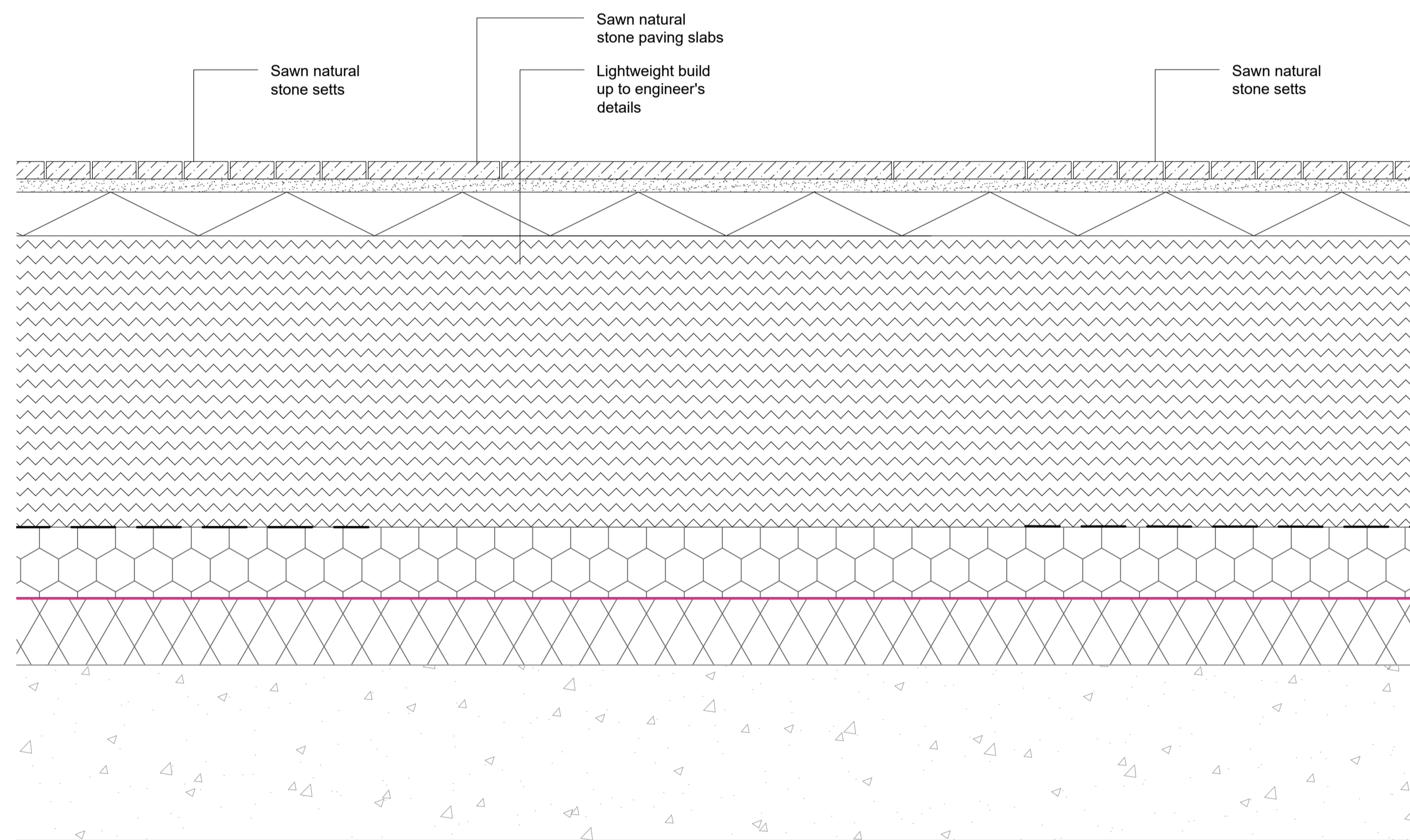
01 Stone slab and sett paving 301 1:10@ A1
