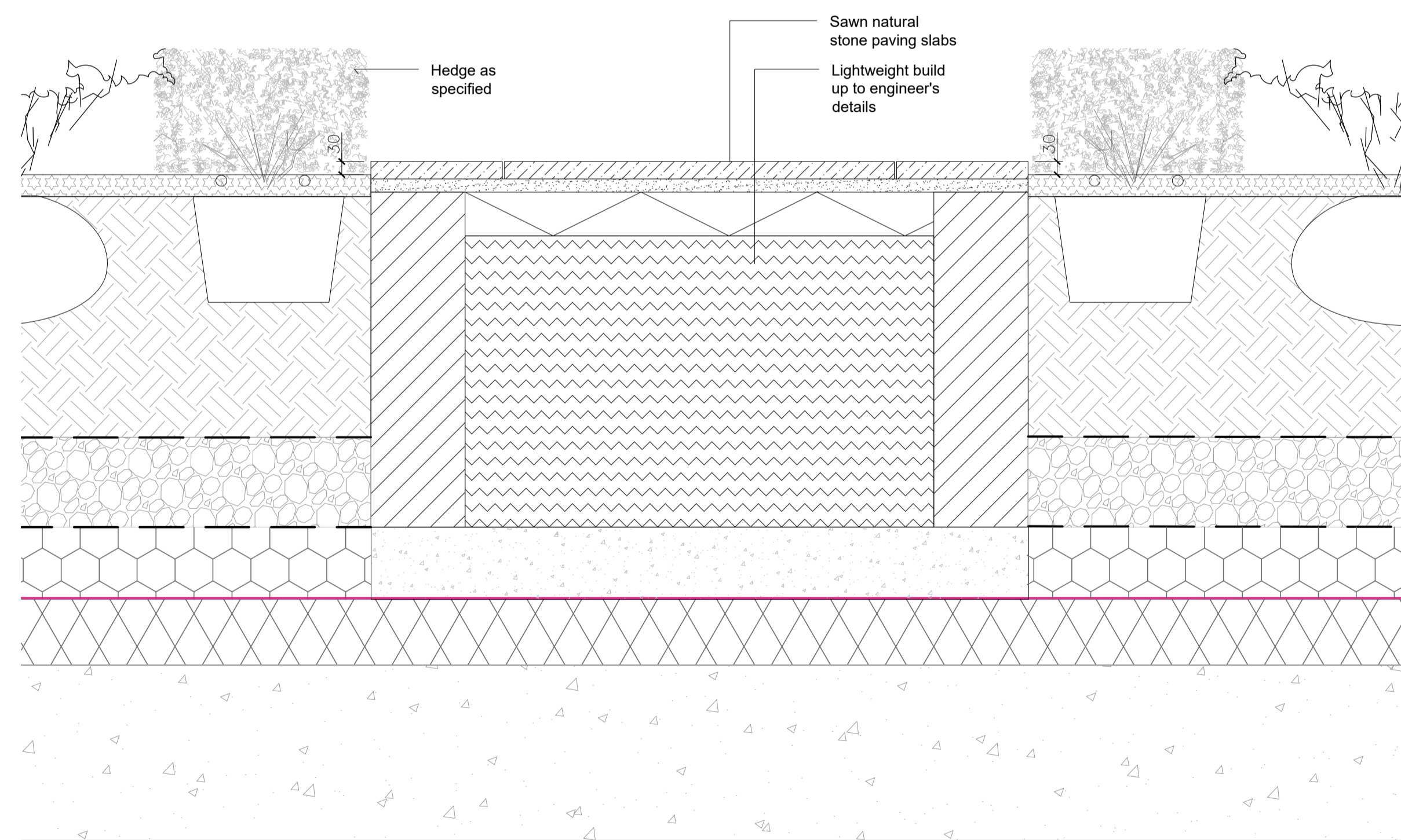
02 Stone slab paving/ hedge interface 301 1:10@ A1
