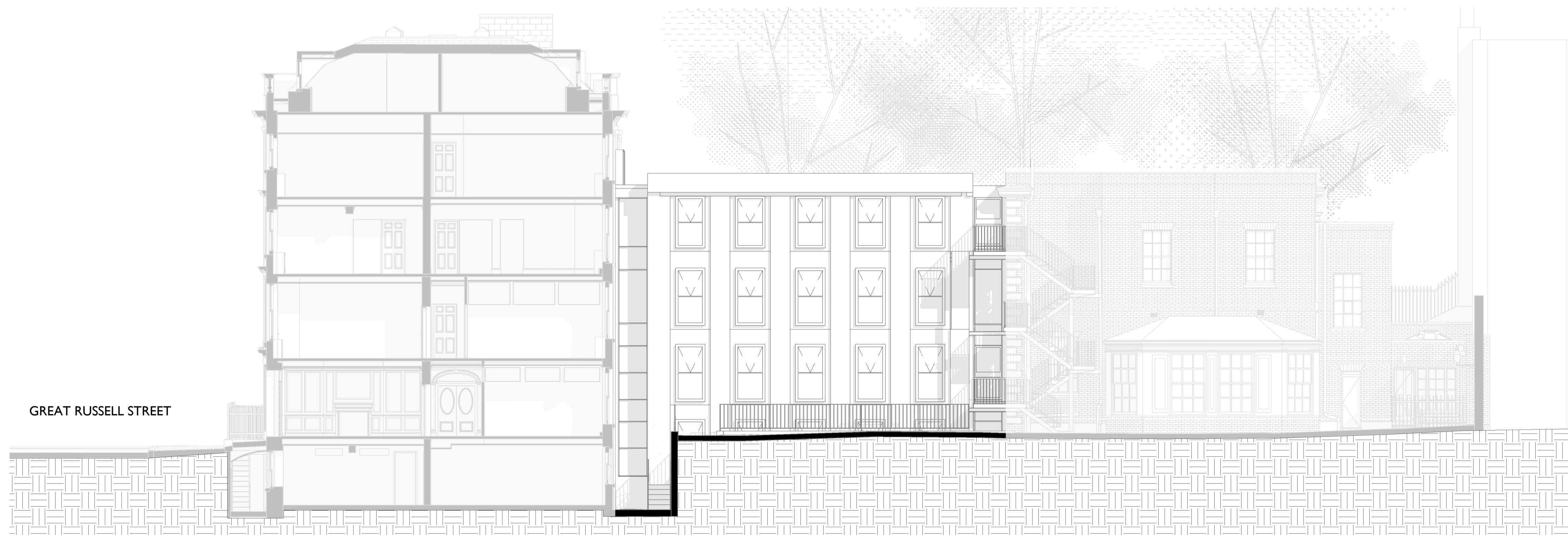
Proposed Rear Long Elevation 1 : 100
