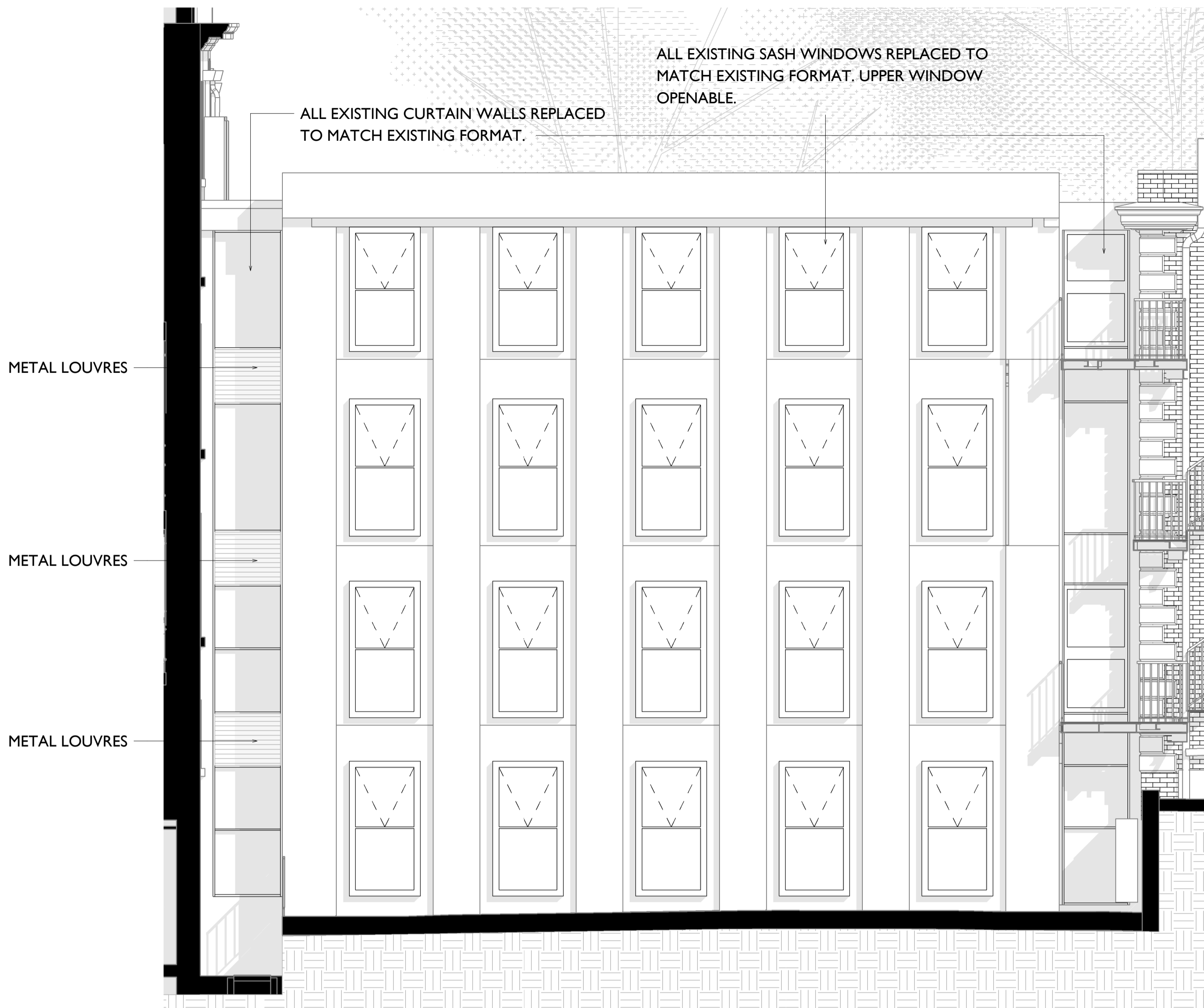
Proposed NE Elevation 1 : 50
