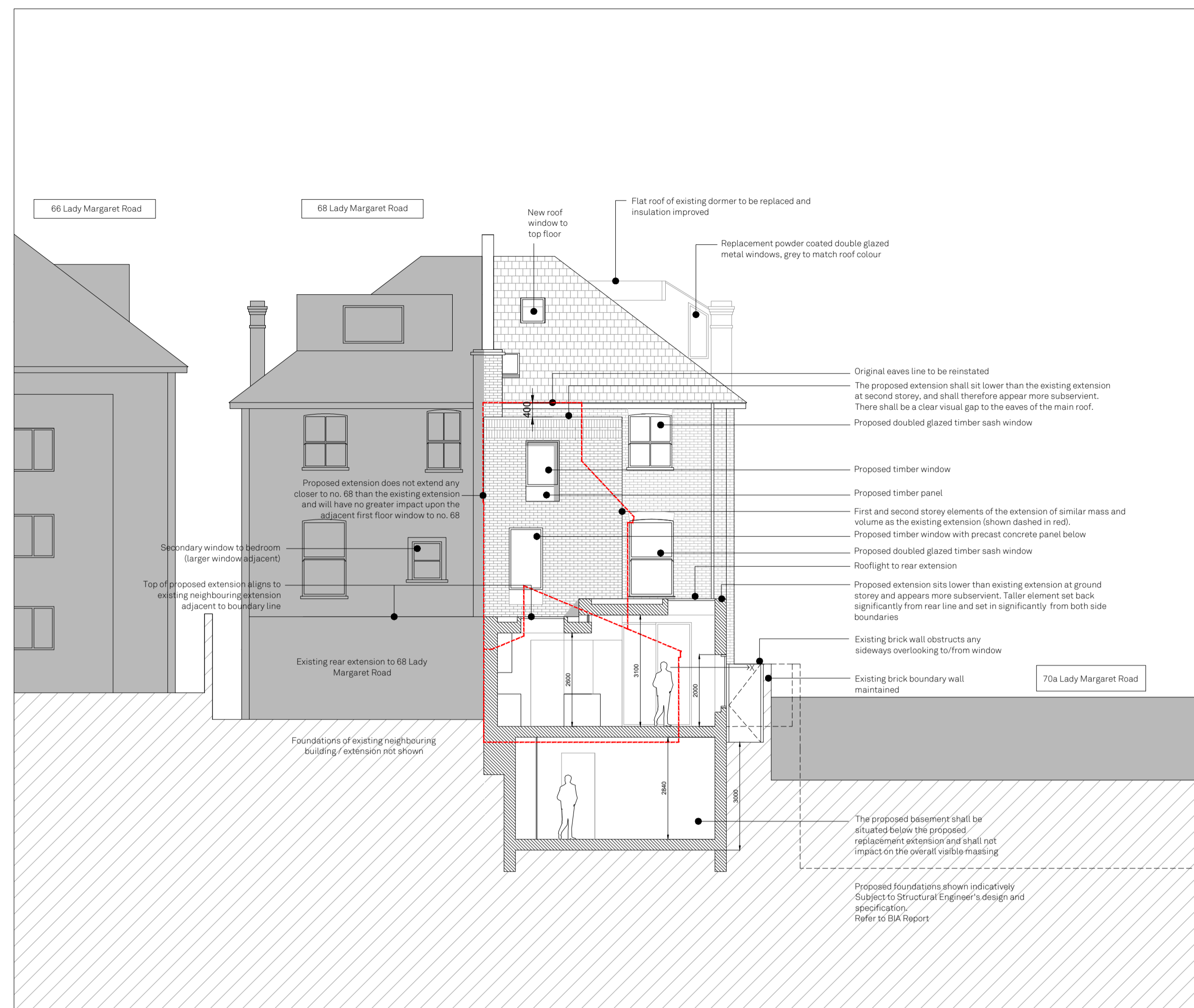
02 - PROPOSED SHORT SECTION
