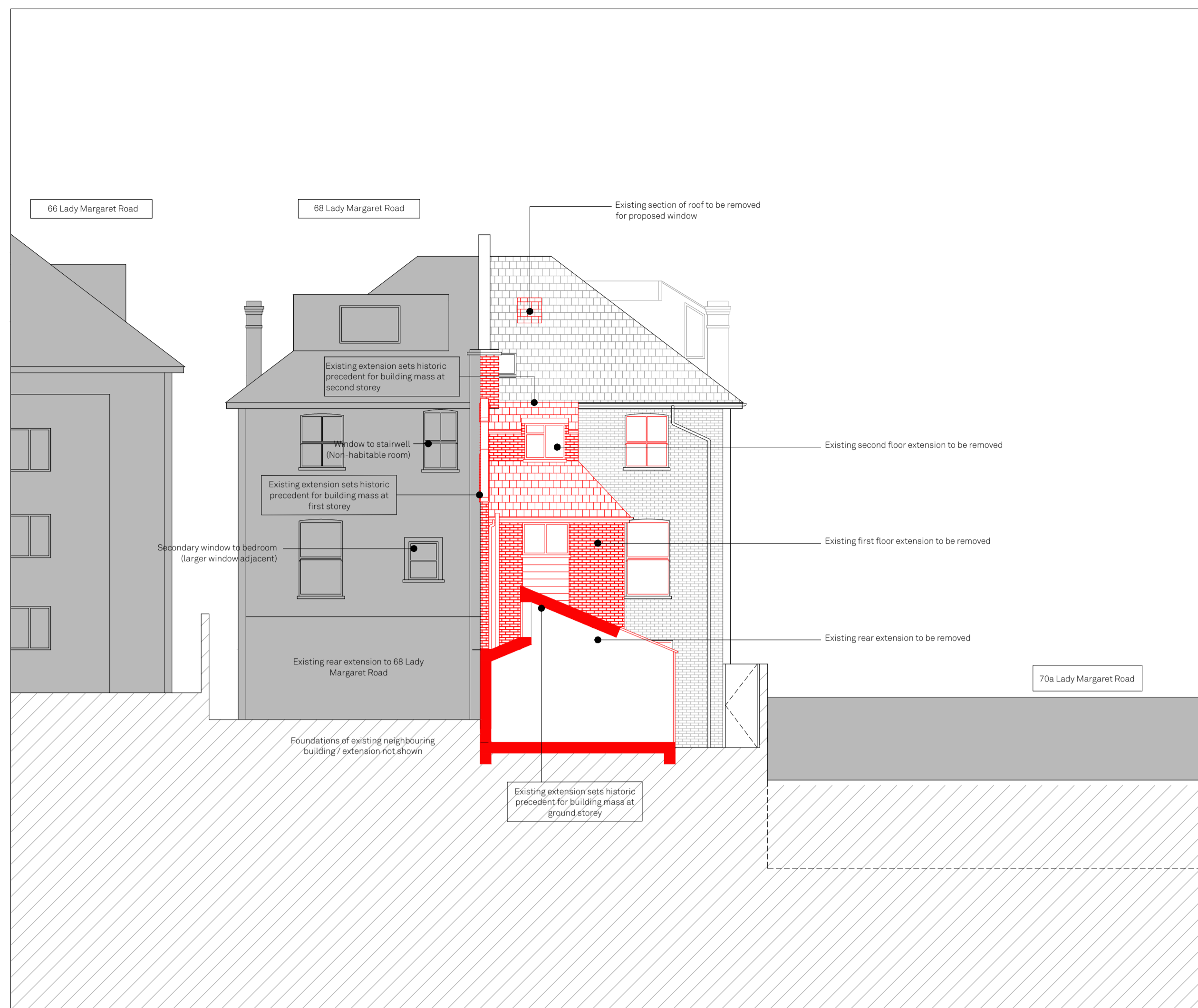
01 - EXISTING SHORT SECTION
