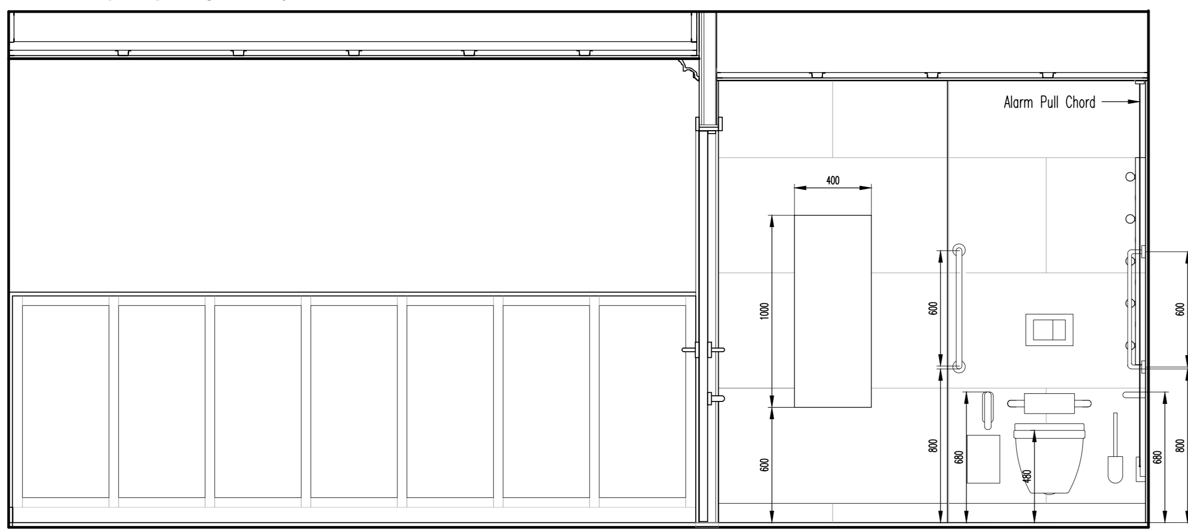
ELEVATION E - SCALE 1:20
