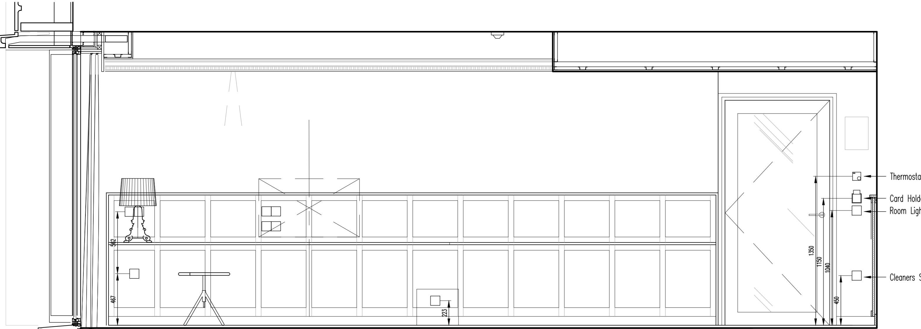
ELEVATION C - SCALE 1:20
