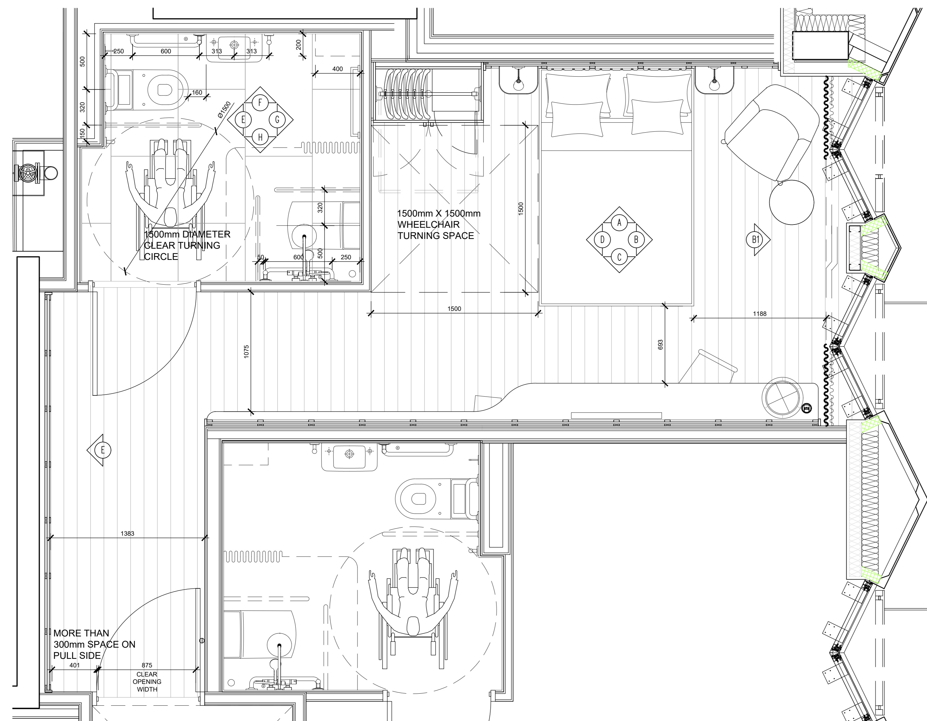
FIRST FLOOR EXTRACT - SCALE 1:20
