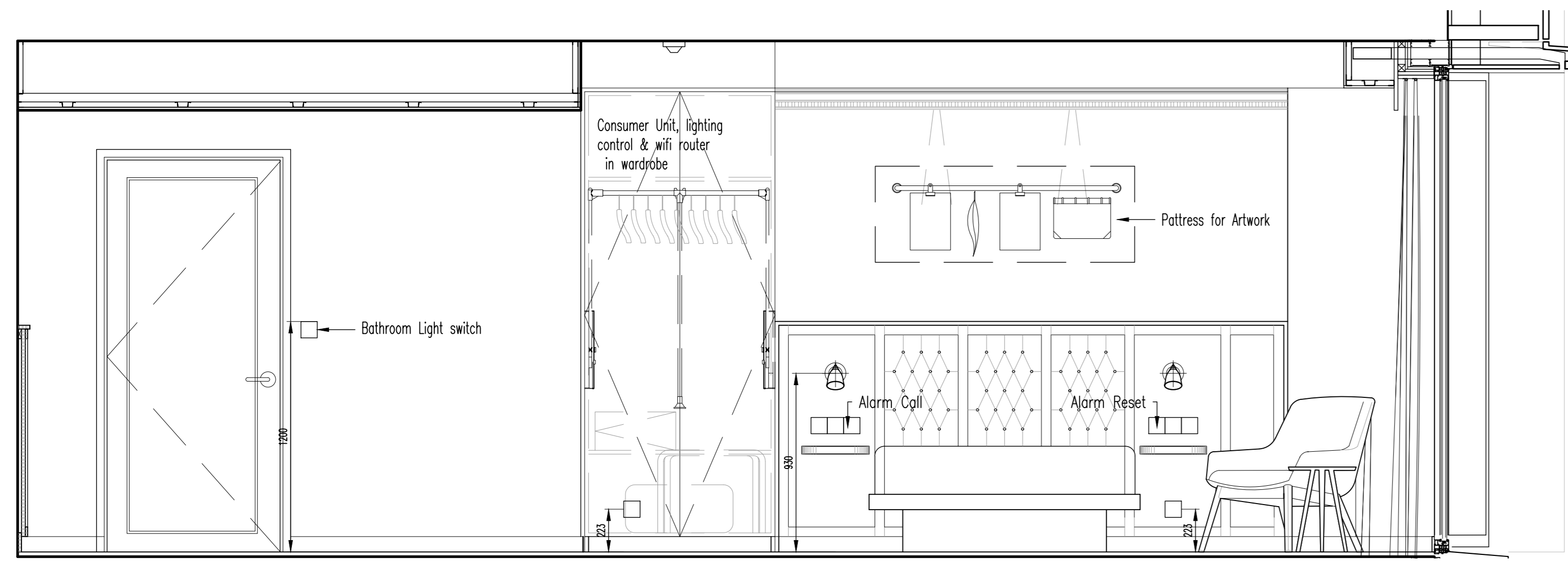
ELEVATION A - SCALE 1:20
