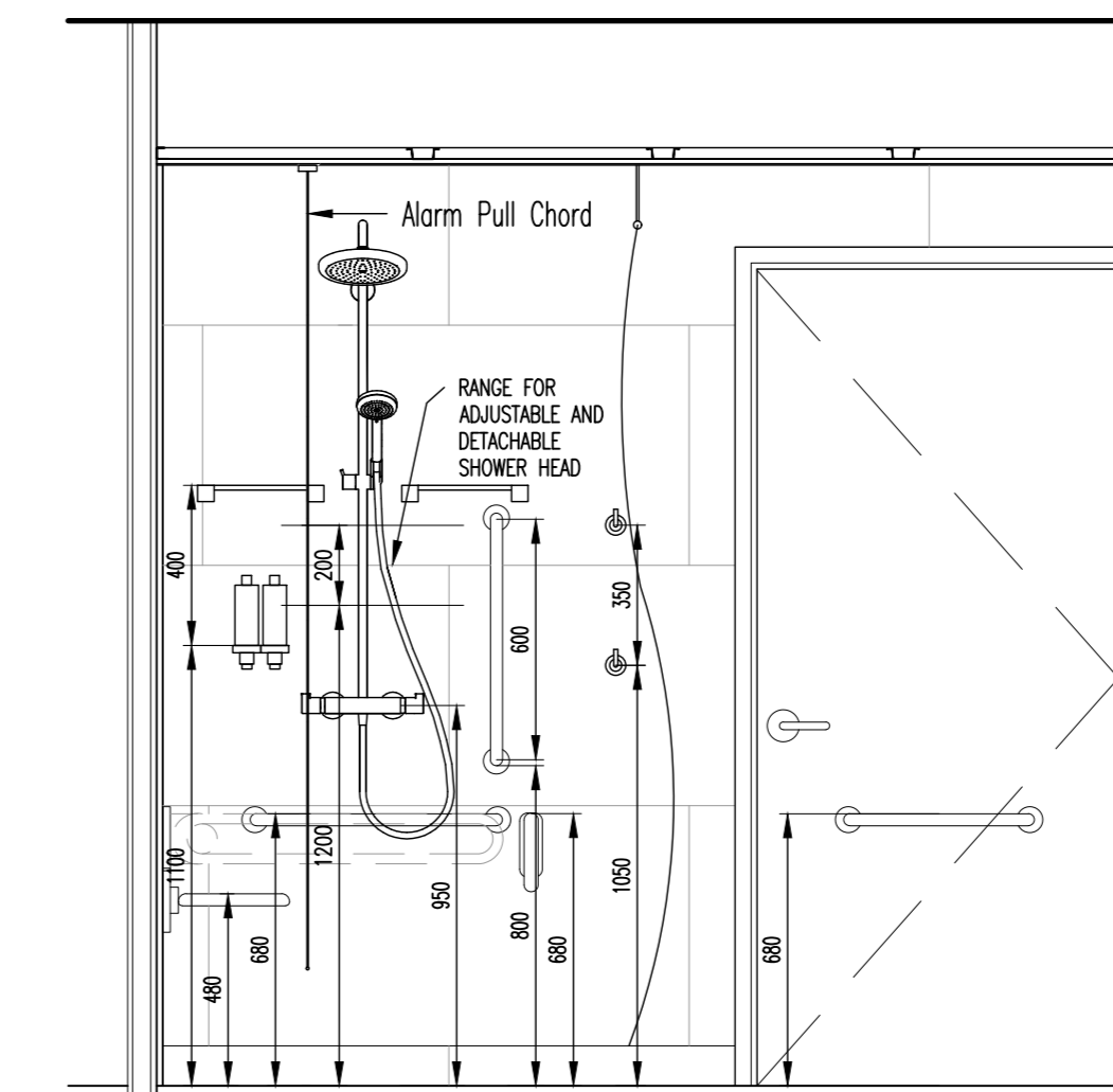
ELEVATION H - SCALE 1:20
